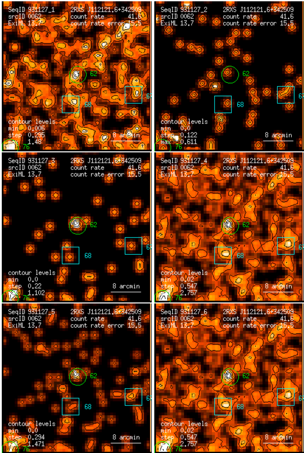
Figure 62: RASS 931127: detection 0062: band rate images, Gaussian filter: (1) PSPC channels 11 – 41, (2) 52 – 90, (3) 91 – 201, (4) 11 – 235, (5) 52 – 201, (6) 11 – 201. Broad band rates in counts/ks. Band rate contour levels in counts/ks/arcmin 2 .
