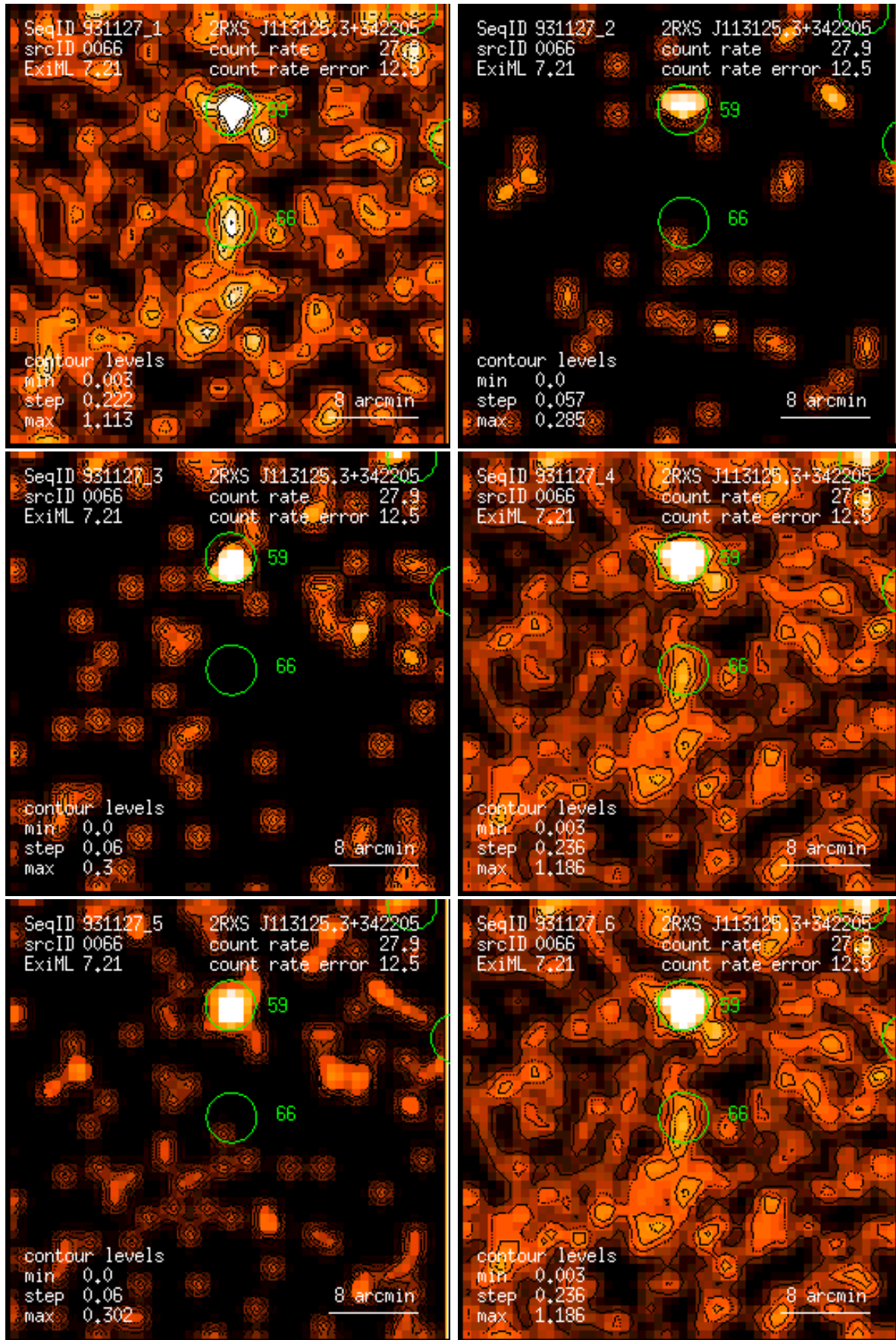
Figure 66: RASS 931127: detection 0066: band rate images, Gaussian filter: (1) PSPC channels 11 – 41, (2) 52 – 90, (3) 91 – 201, (4) 11 – 235, (5) 52 – 201, (6) 11 – 201. Broad band rates in counts/ks. Band rate contour levels in counts/ks/arcmin 2 .
