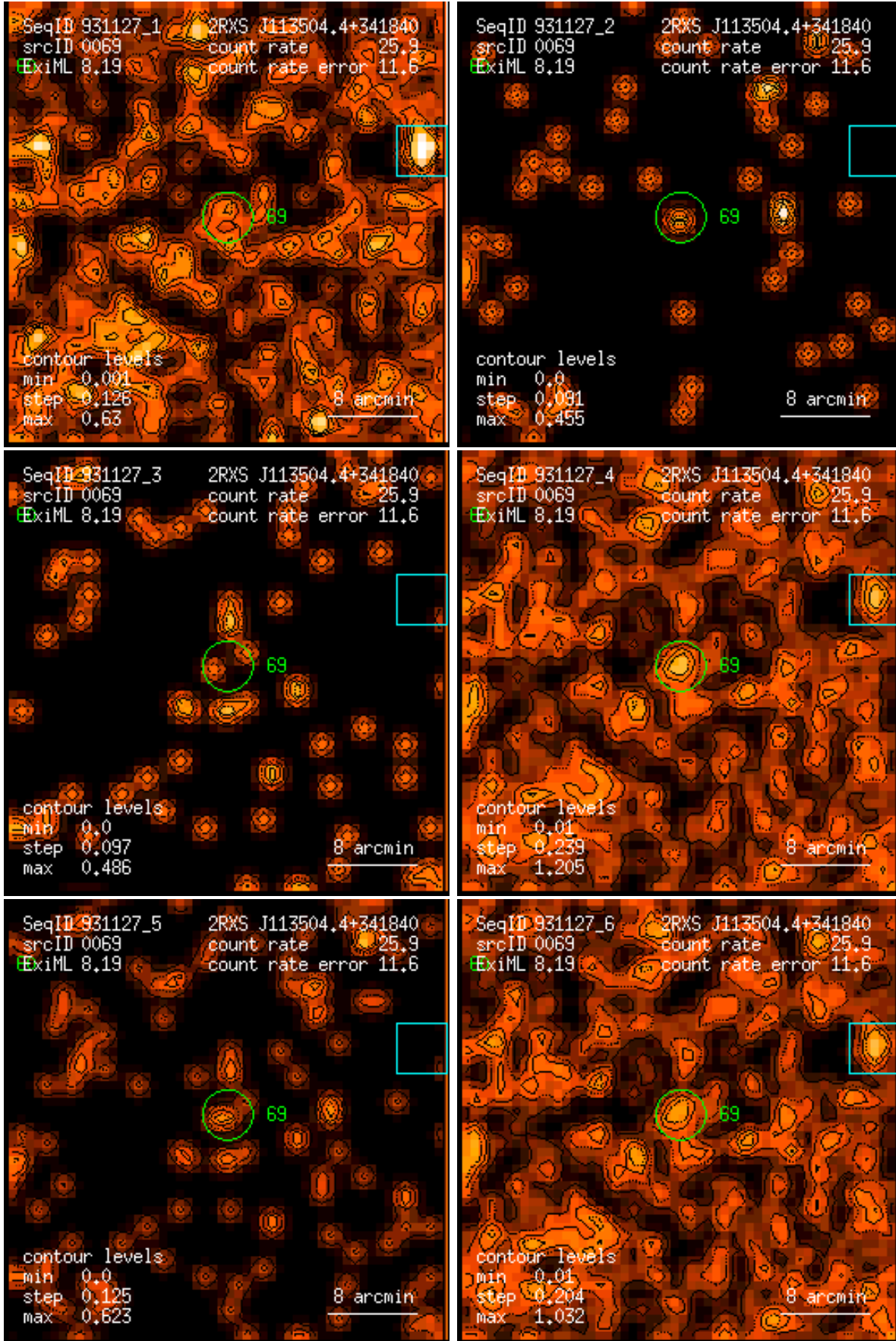
Figure 69: RASS 931127: detection 0069: band rate images, Gaussian filter: (1) PSPC channels 11 – 41, (2) 52 – 90, (3) 91 – 201, (4) 11 – 235, (5) 52 – 201, (6) 11 – 201. Broad band rates in counts/ks. Band rate contour levels in counts/ks/arcmin 2 .
