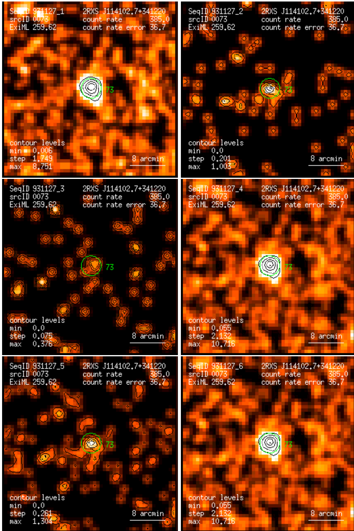
Figure 73: RASS 931127: detection 0073: band rate images, Gaussian filter: (1) PSPC channels 11 – 41, (2) 52 – 90, (3) 91 – 201, (4) 11 – 235, (5) 52 – 201, (6) 11 – 201. Broad band rates in counts/ks. Band rate contour levels in counts/ks/arcmin 2 .
