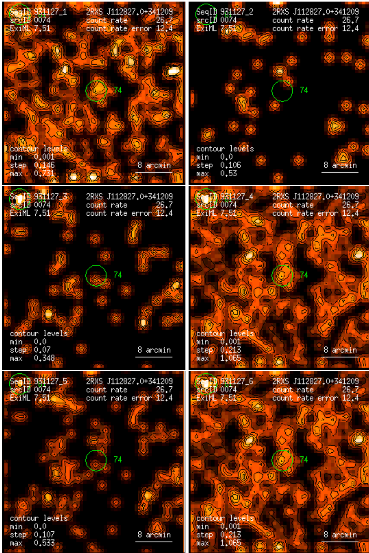
Figure 74: RASS 931127: detection 0074: band rate images, Gaussian filter: (1) PSPC channels 11 – 41, (2) 52 – 90, (3) 91 – 201, (4) 11 – 235, (5) 52 – 201, (6) 11 – 201. Broad band rates in counts/ks. Band rate contour levels in counts/ks/arcmin 2 .
