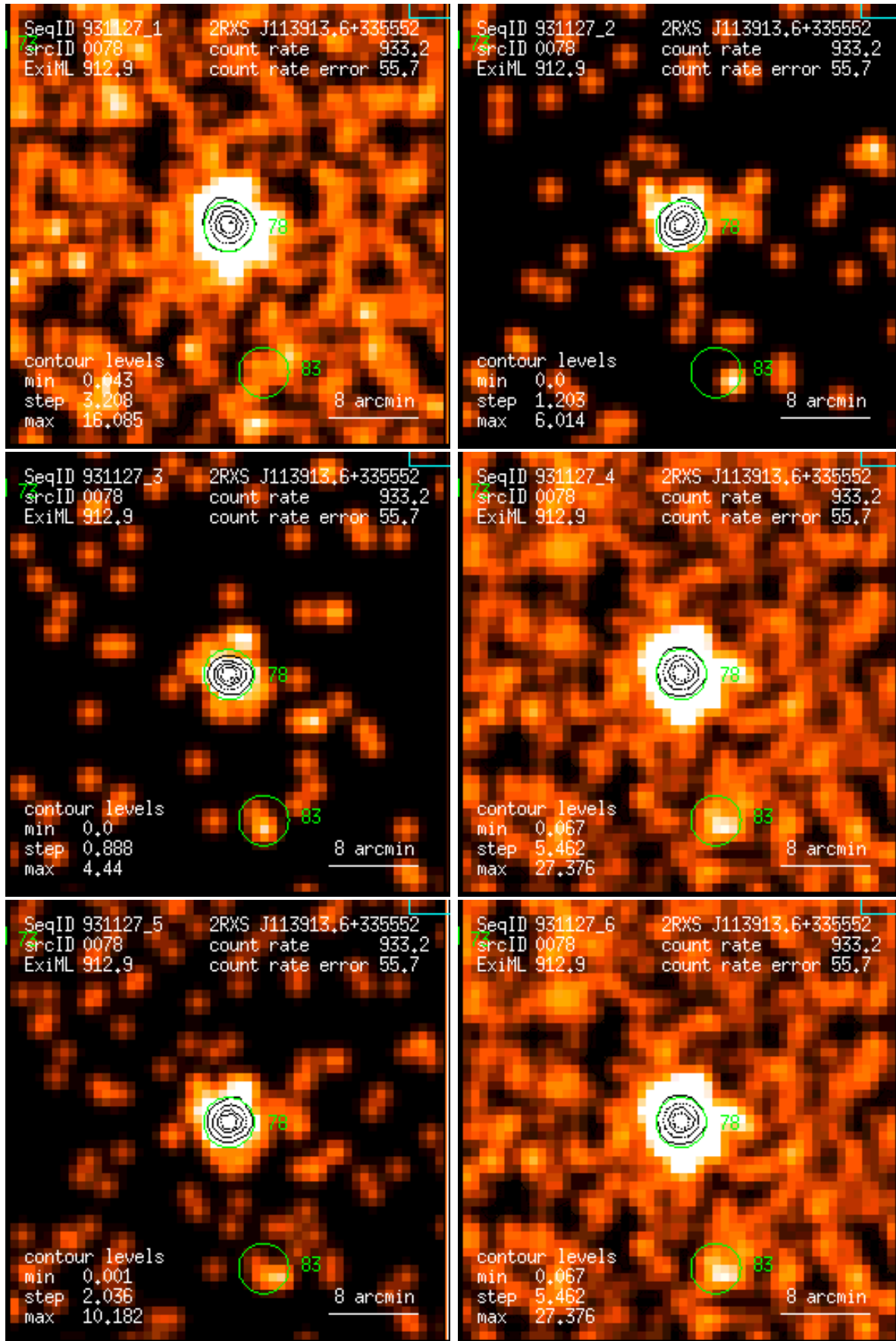
Figure 78: RASS 931127: detection 0078: band rate images, Gaussian filter: (1) PSPC channels 11 – 41, (2) 52 – 90, (3) 91 – 201, (4) 11 – 235, (5) 52 – 201, (6) 11 – 201. Broad band rates in counts/ks. Band rate contour levels in counts/ks/arcmin 2 .
