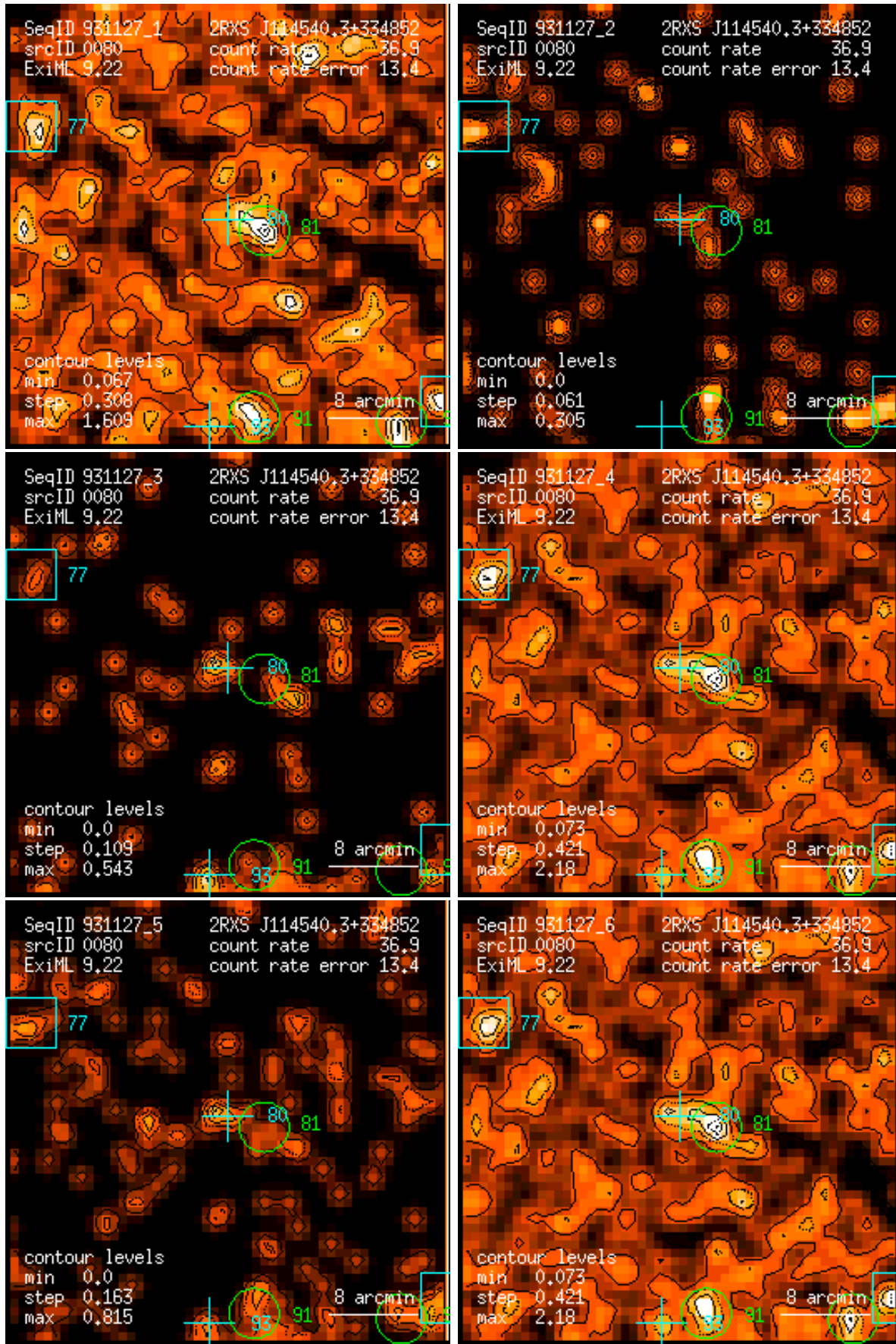
Figure 80: RASS 931127: detection 0080: band rate images, Gaussian filter: (1) PSPC channels 11 – 41, (2) 52 – 90, (3) 91 – 201, (4) 11 – 235, (5) 52 – 201, (6) 11 – 201. Broad band rates in counts/ks. Band rate contour levels in counts/ks/arcmin 2 .
