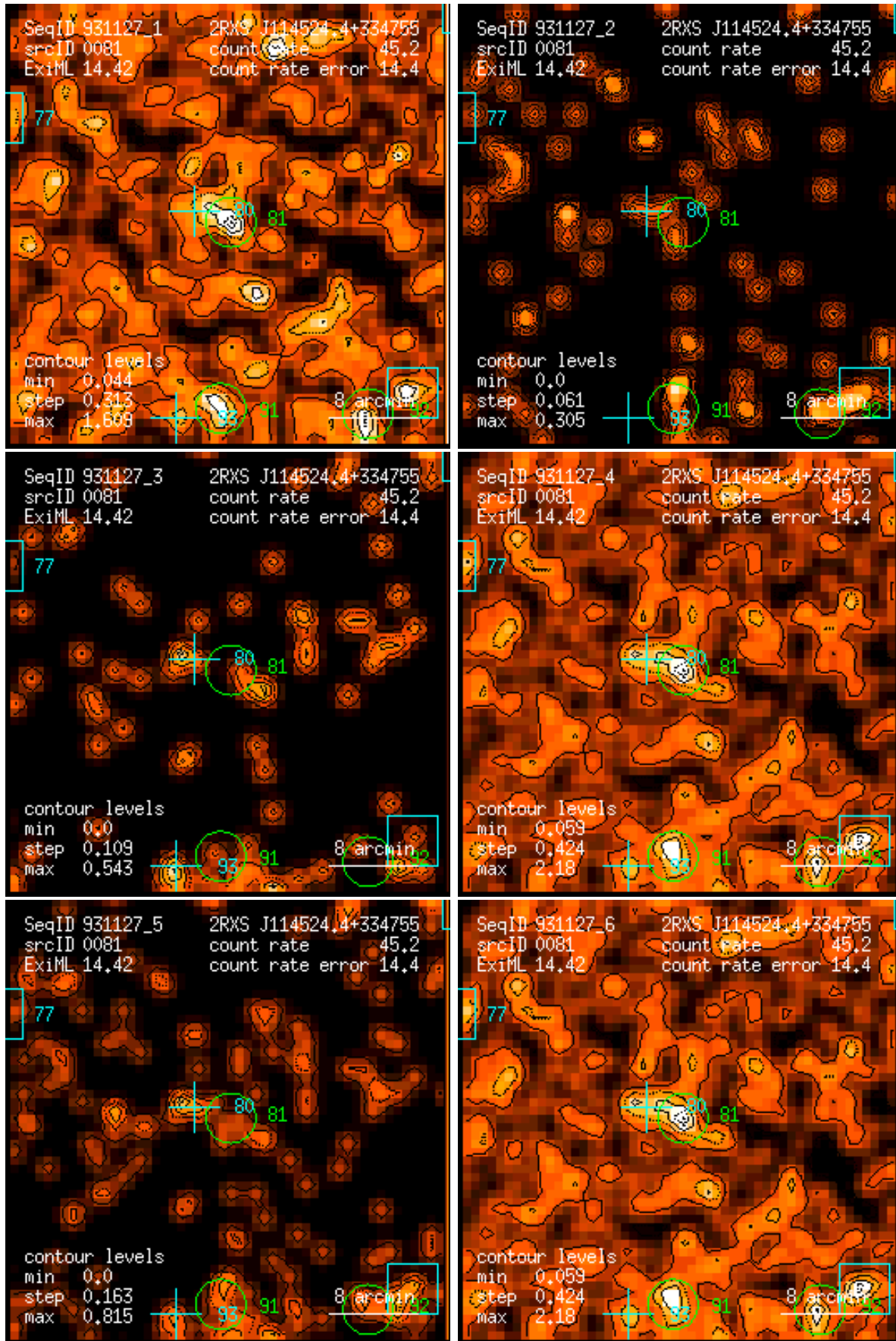
Figure 81: RASS 931127: detection 0081: band rate images, Gaussian filter: (1) PSPC channels 11 – 41, (2) 52 – 90, (3) 91 – 201, (4) 11 – 235, (5) 52 – 201, (6) 11 – 201. Broad band rates in counts/ks. Band rate contour levels in counts/ks/arcmin 2 .
