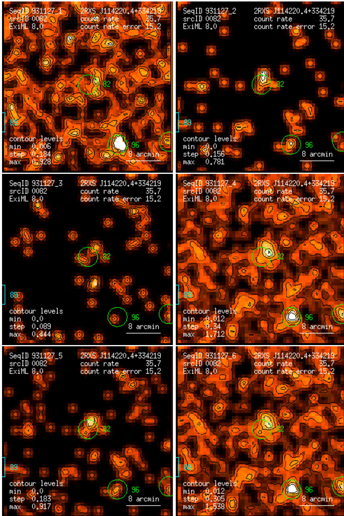
Figure 82: RASS 931127: detection 0082: band rate images, Gaussian filter: (1) PSPC channels 11 – 41, (2) 52 – 90, (3) 91 – 201, (4) 11 – 235, (5) 52 – 201, (6) 11 – 201. Broad band rates in counts/ks. Band rate contour levels in counts/ks/arcmin 2 .
