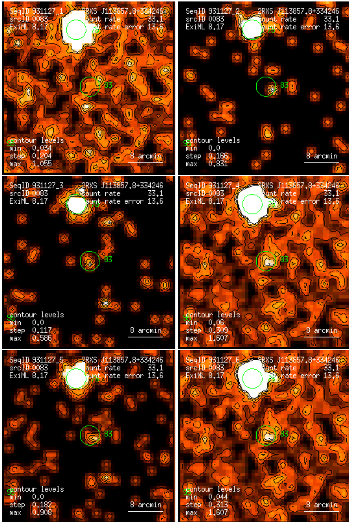
Figure 83: RASS 931127: detection 0083: band rate images, Gaussian filter: (1) PSPC channels 11 – 41, (2) 52 – 90, (3) 91 – 201, (4) 11 – 235, (5) 52 – 201, (6) 11 – 201. Broad band rates in counts/ks. Band rate contour levels in counts/ks/arcmin 2 .
