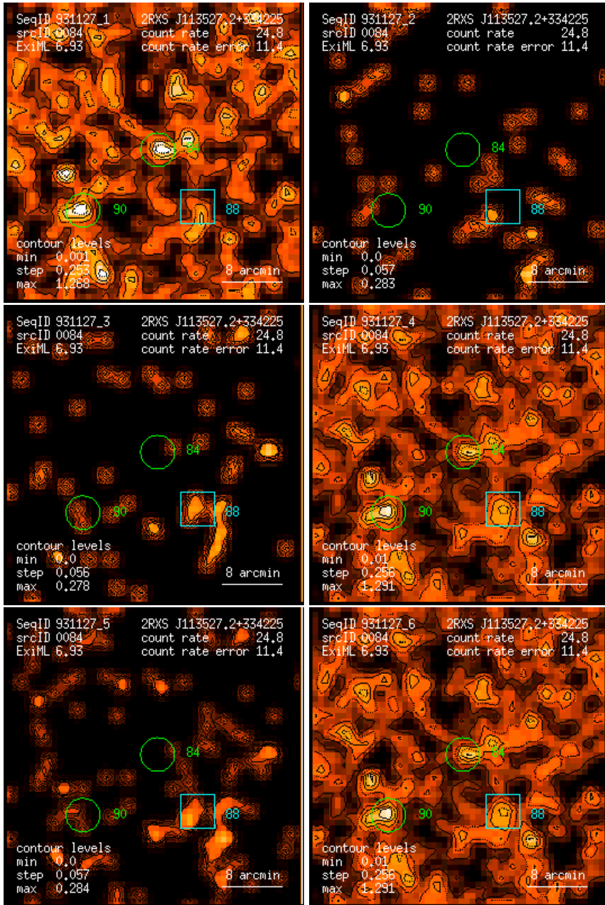
Figure 84: RASS 931127: detection 0084: band rate images, Gaussian filter: (1) PSPC channels 11 – 41, (2) 52 – 90, (3) 91 – 201, (4) 11 – 235, (5) 52 – 201, (6) 11 – 201. Broad band rates in counts/ks. Band rate contour levels in counts/ks/arcmin 2 .
