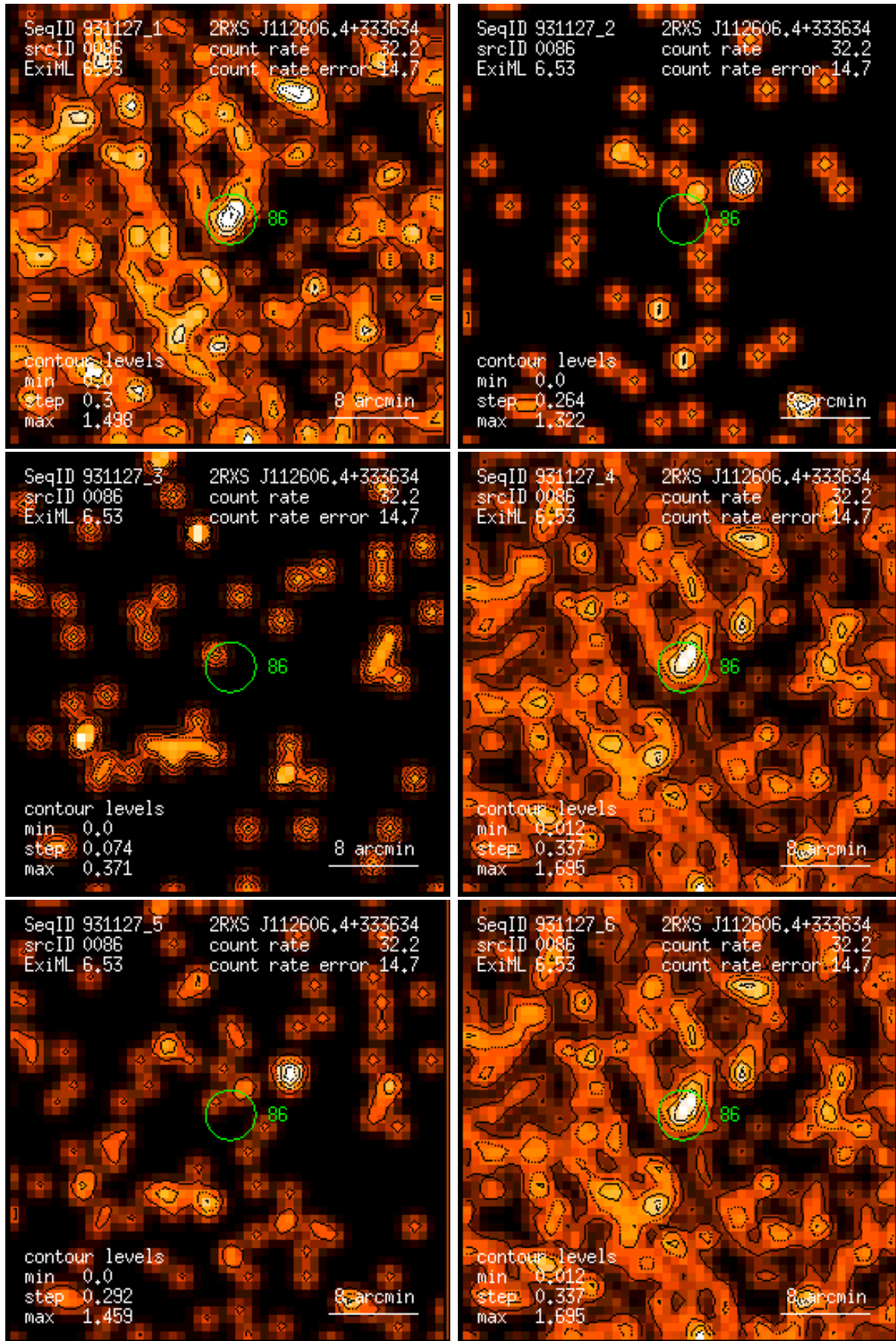
Figure 86: RASS 931127: detection 0086: band rate images, Gaussian filter: (1) PSPC channels 11 – 41, (2) 52 – 90, (3) 91 – 201, (4) 11 – 235, (5) 52 – 201, (6) 11 – 201. Broad band rates in counts/ks. Band rate contour levels in counts/ks/arcmin 2 .
