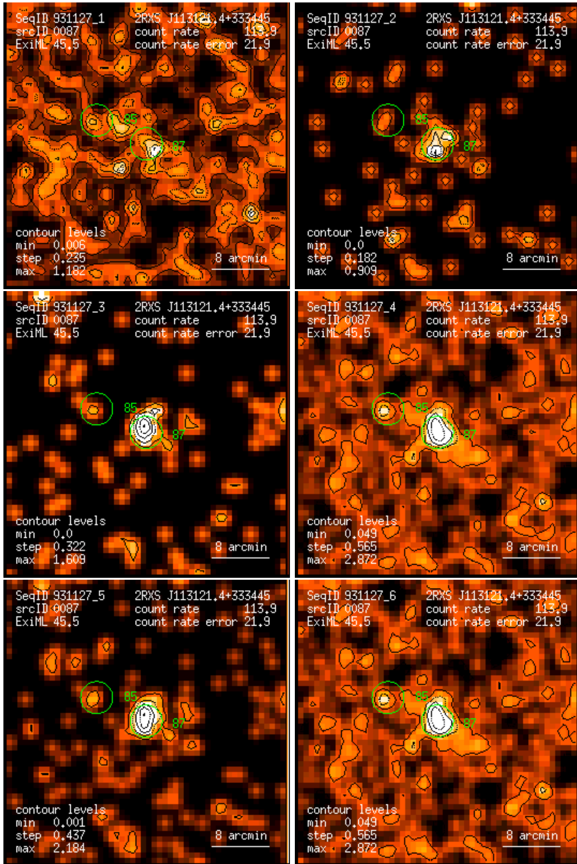
Figure 87: RASS 931127: detection 0087: band rate images, Gaussian filter: (1) PSPC channels 11 – 41, (2) 52 – 90, (3) 91 – 201, (4) 11 – 235, (5) 52 – 201, (6) 11 – 201. Broad band rates in counts/ks. Band rate contour levels in counts/ks/arcmin 2 .
