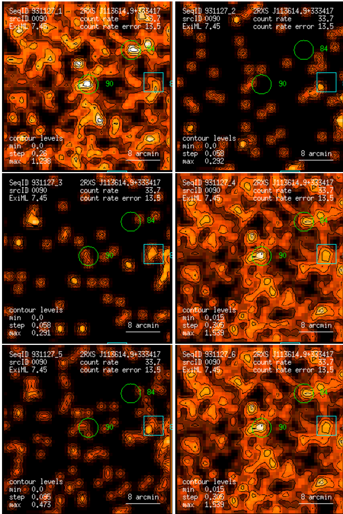
Figure 90: RASS 931127: detection 0090: band rate images, Gaussian filter: (1) PSPC channels 11 – 41, (2) 52 – 90, (3) 91 – 201, (4) 11 – 235, (5) 52 – 201, (6) 11 – 201. Broad band rates in counts/ks. Band rate contour levels in counts/ks/arcmin 2 .
