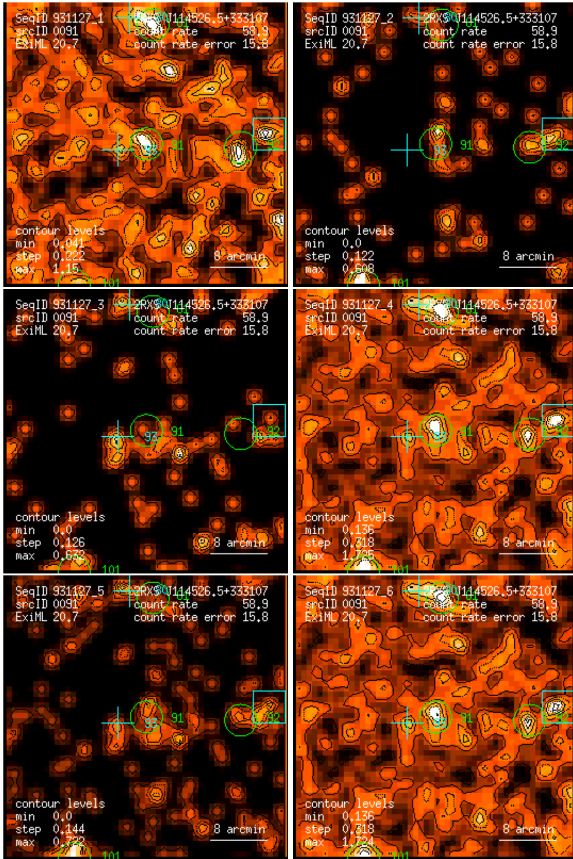
Figure 91: RASS 931127: detection 0091: band rate images, Gaussian filter: (1) PSPC channels 11 – 41, (2) 52 – 90, (3) 91 – 201, (4) 11 – 235, (5) 52 – 201, (6) 11 – 201. Broad band rates in counts/ks. Band rate contour levels in counts/ks/arcmin 2 .
