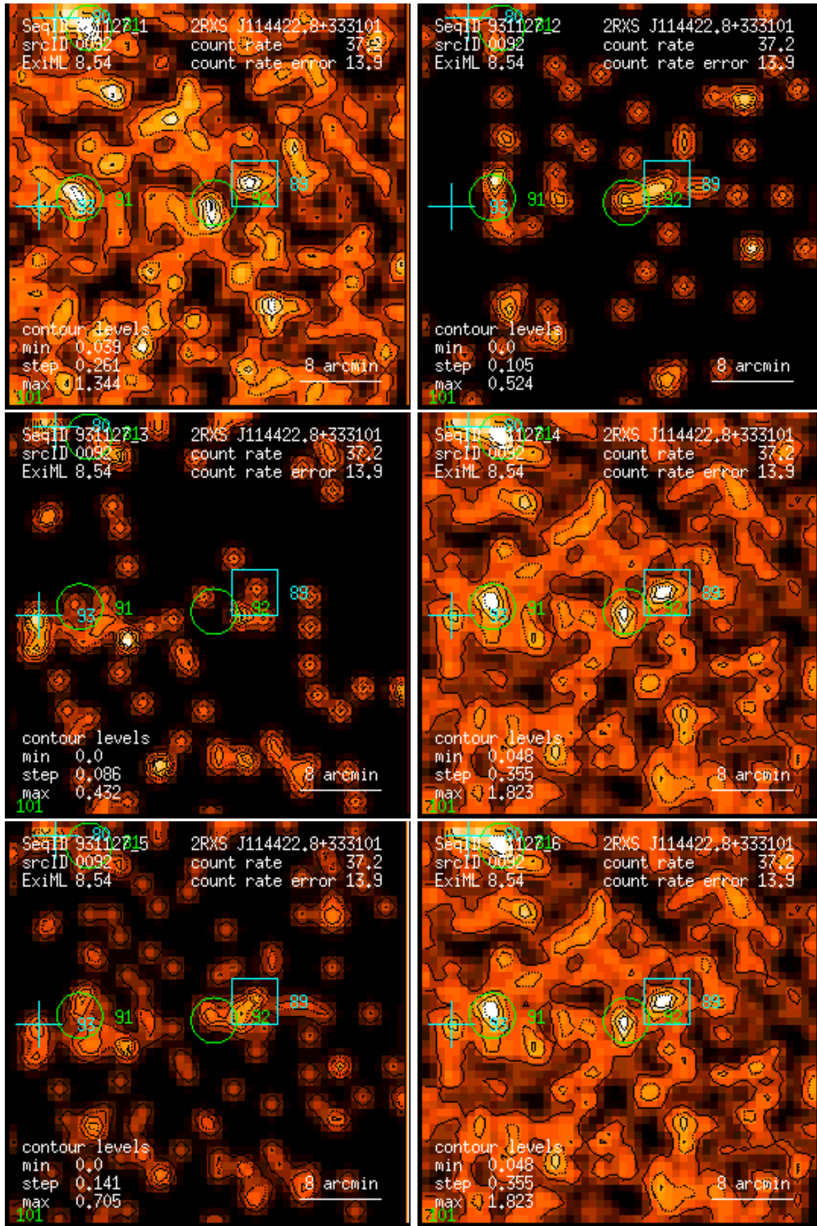
Figure 92: RASS 931127: detection 0092: band rate images, Gaussian filter: (1) PSPC channels 11 – 41, (2) 52 – 90, (3) 91 – 201, (4) 11 – 235, (5) 52 – 201, (6) 11 – 201. Broad band rates in counts/ks. Band rate contour levels in counts/ks/arcmin 2 .
