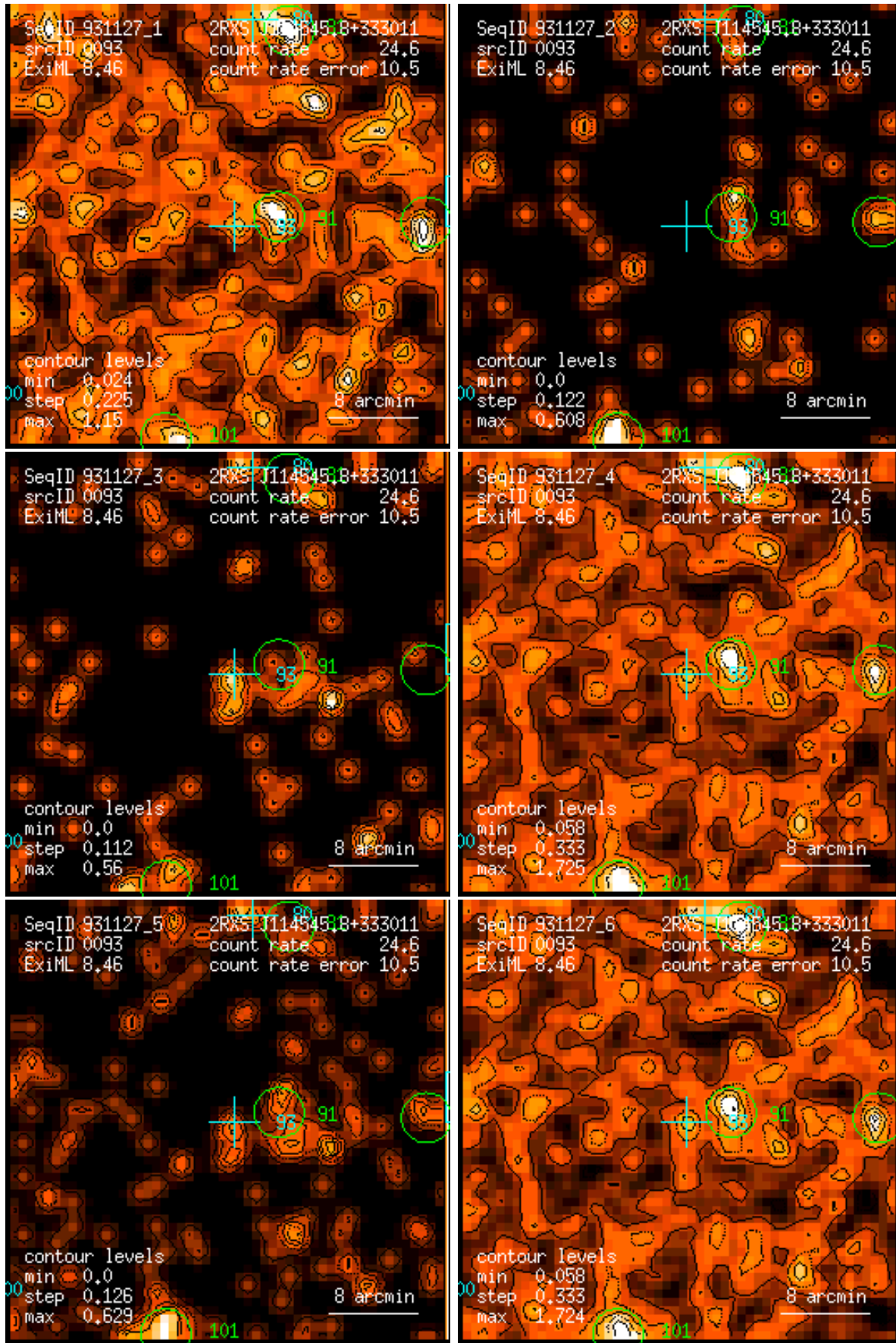
Figure 93: RASS 931127: detection 0093: band rate images, Gaussian filter: (1) PSPC channels 11 – 41, (2) 52 – 90, (3) 91 – 201, (4) 11 – 235, (5) 52 – 201, (6) 11 – 201. Broad band rates in counts/ks. Band rate contour levels in counts/ks/arcmin 2 .
