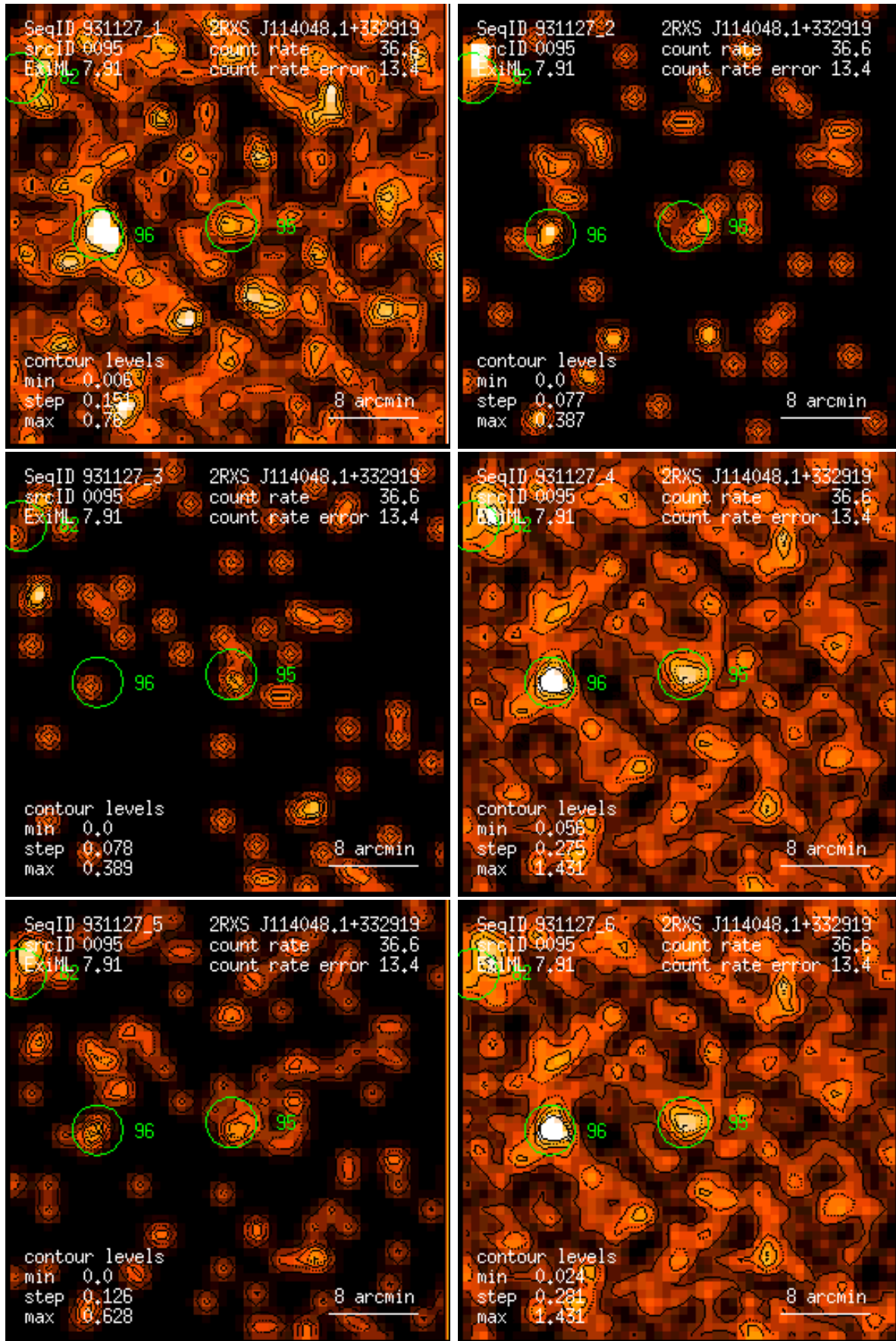
Figure 95: RASS 931127: detection 0095: band rate images, Gaussian filter: (1) PSPC channels 11 – 41, (2) 52 – 90, (3) 91 – 201, (4) 11 – 235, (5) 52 – 201, (6) 11 – 201. Broad band rates in counts/ks. Band rate contour levels in counts/ks/arcmin 2 .
