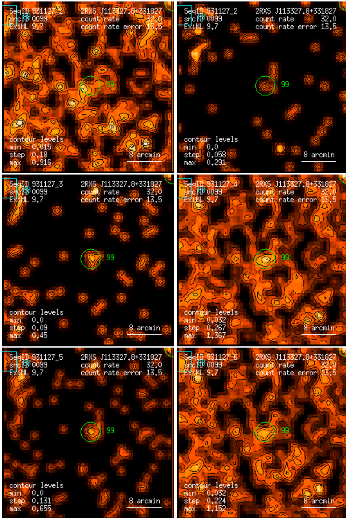
Figure 99: RASS 931127: detection 0099: band rate images, Gaussian filter: (1) PSPC channels 11 – 41, (2) 52 – 90, (3) 91 – 201, (4) 11 – 235, (5) 52 – 201, (6) 11 – 201. Broad band rates in counts/ks. Band rate contour levels in counts/ks/arcmin 2 .
