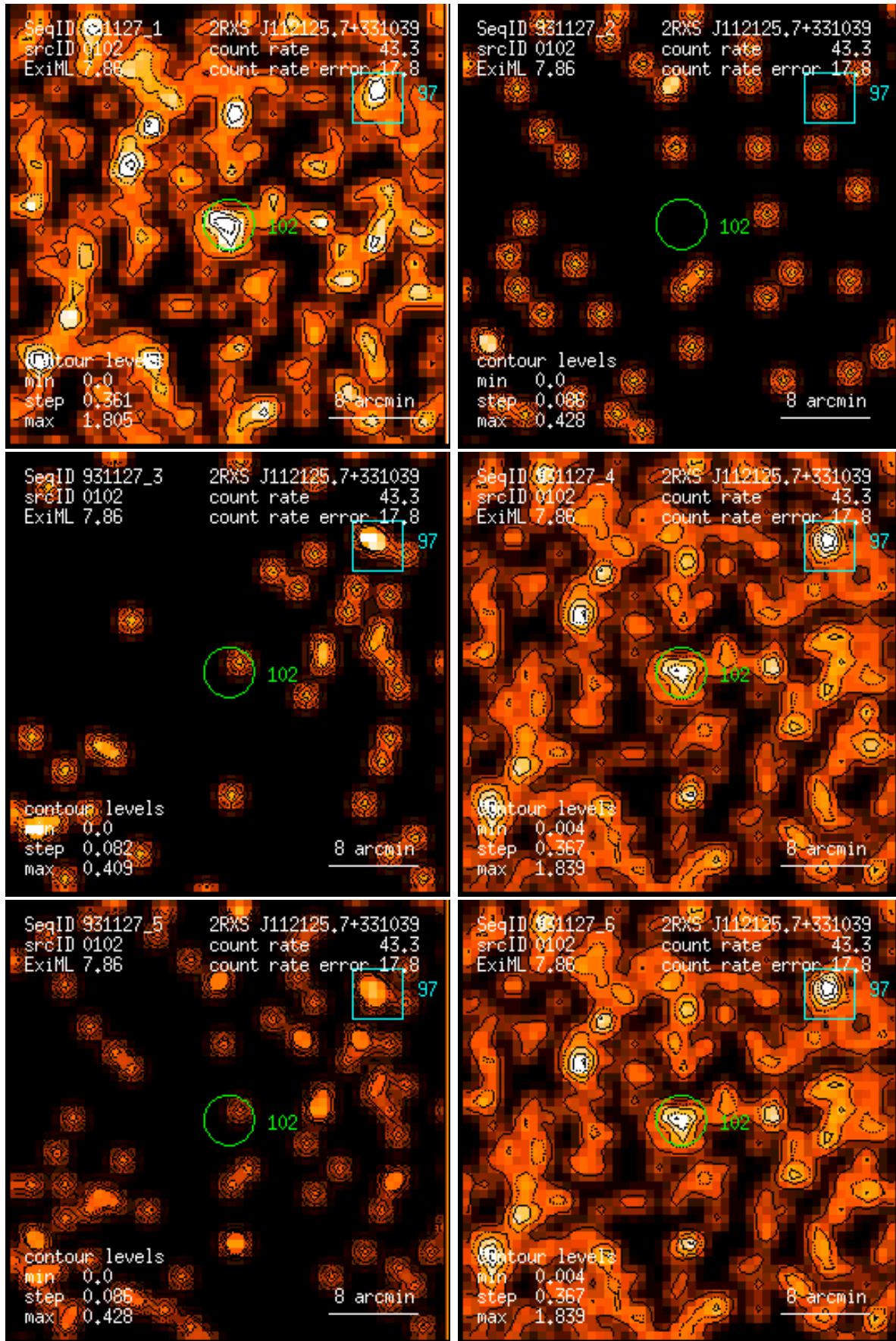
Figure 102: RASS 931127: detection 0102: band rate images, Gaussian filter: (1) PSPC channels 11 – 41, (2) 52 – 90, (3) 91 – 201, (4) 11 – 235, (5) 52 – 201, (6) 11 – 201. Broad band rates in counts/ks. Band rate contour levels in counts/ks/arcmin 2 .
