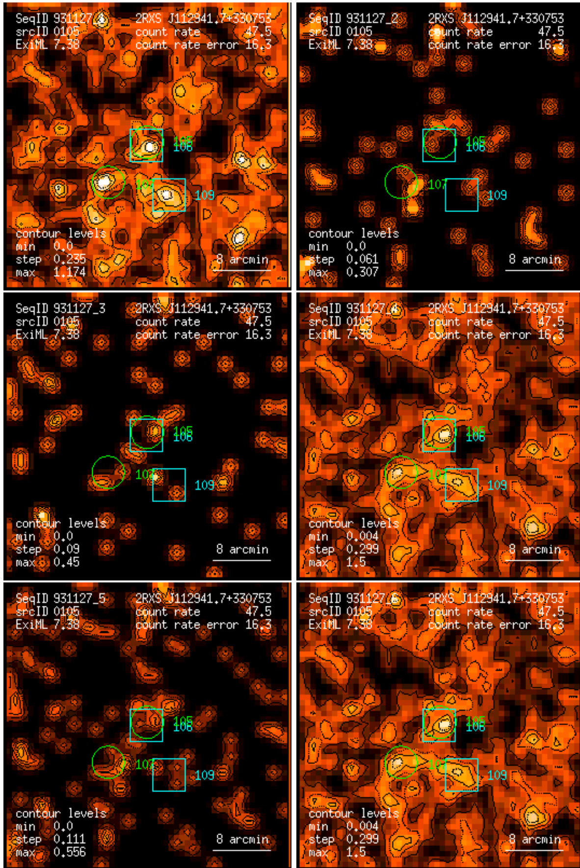
Figure 105: RASS 931127: detection 0105: band rate images, Gaussian filter: (1) PSPC channels 11 – 41, (2) 52 – 90, (3) 91 – 201, (4) 11 – 235, (5) 52 – 201, (6) 11 – 201. Broad band rates in counts/ks. Band rate contour levels in counts/ks/arcmin 2 .
