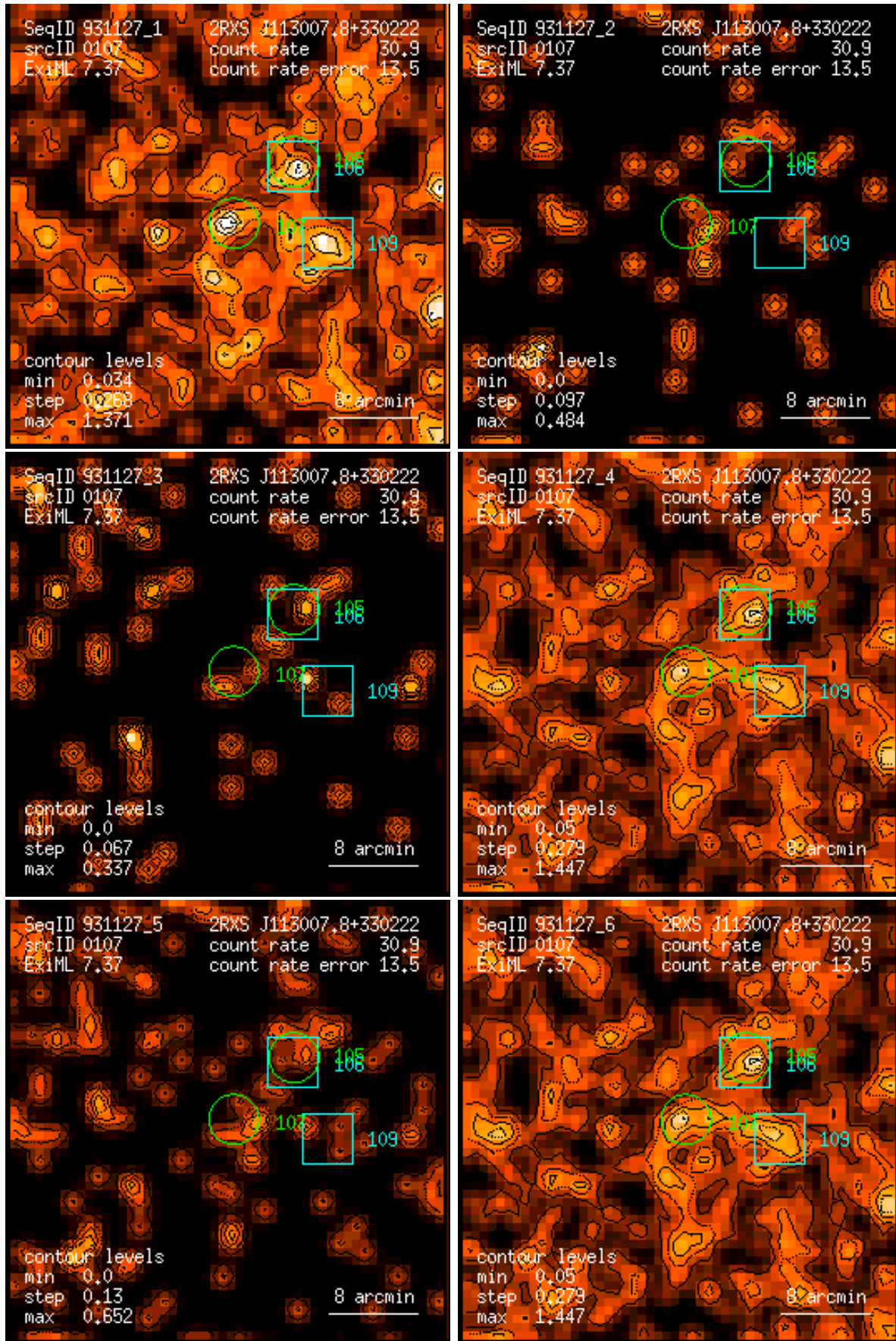
Figure 107: RASS 931127: detection 0107: band rate images, Gaussian filter: (1) PSPC channels 11 – 41, (2) 52 – 90, (3) 91 – 201, (4) 11 – 235, (5) 52 – 201, (6) 11 – 201. Broad band rates in counts/ks. Band rate contour levels in counts/ks/arcmin 2 .
