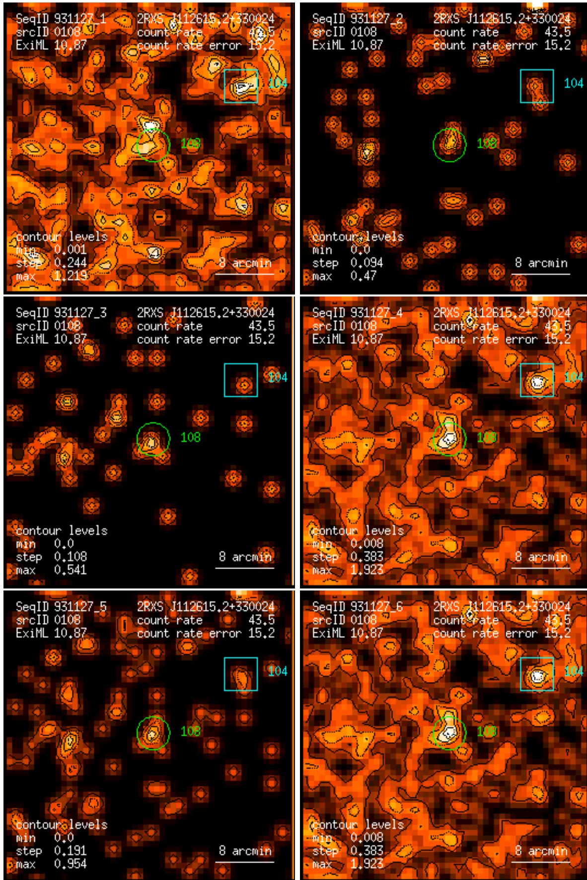
Figure 108: RASS 931127: detection 0108: band rate images, Gaussian filter: (1) PSPC channels 11 – 41, (2) 52 – 90, (3) 91 – 201, (4) 11 – 235, (5) 52 – 201, (6) 11 – 201. Broad band rates in counts/ks. Band rate contour levels in counts/ks/arcmin 2 .
