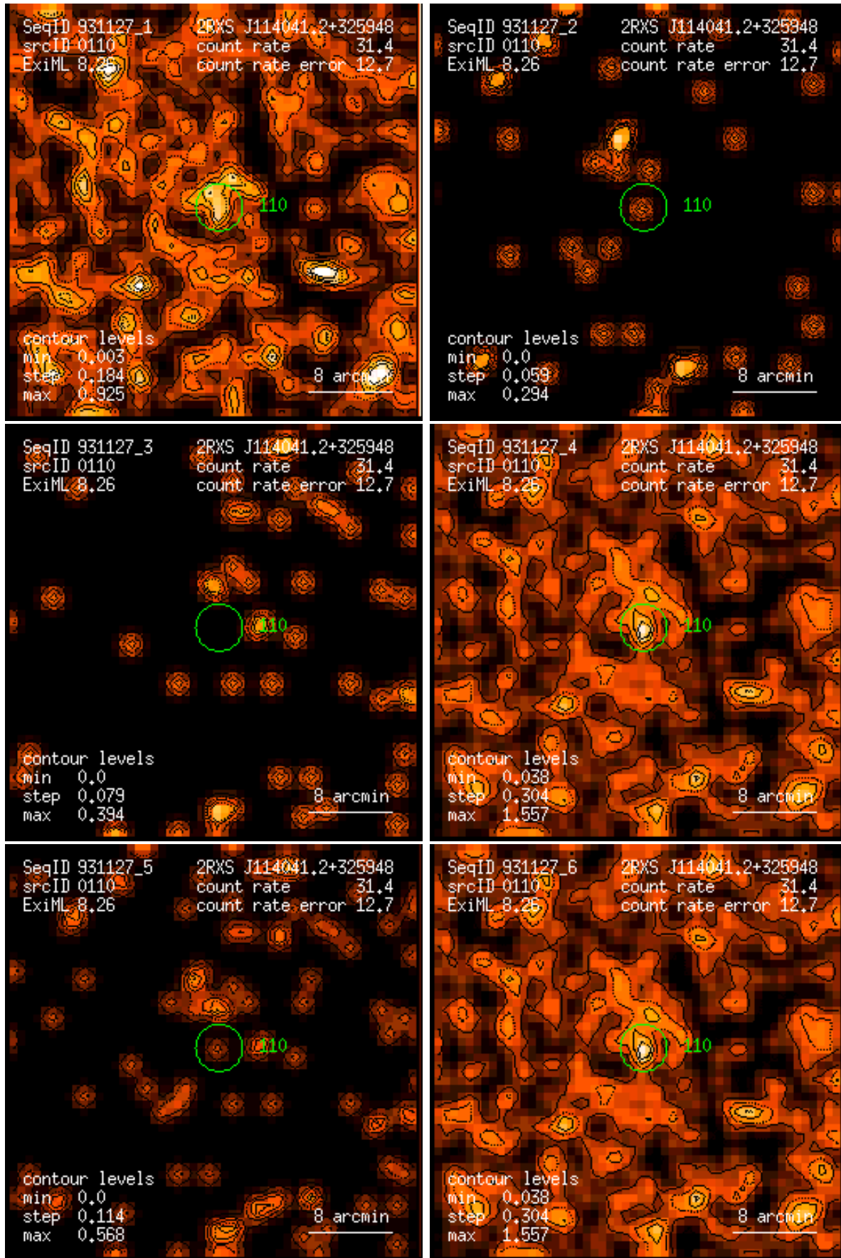
Figure 110: RASS 931127: detection 0110: band rate images, Gaussian filter: (1) PSPC channels 11 – 41, (2) 52 – 90, (3) 91 – 201, (4) 11 – 235, (5) 52 – 201, (6) 11 – 201. Broad band rates in counts/ks. Band rate contour levels in counts/ks/arcmin 2 .
