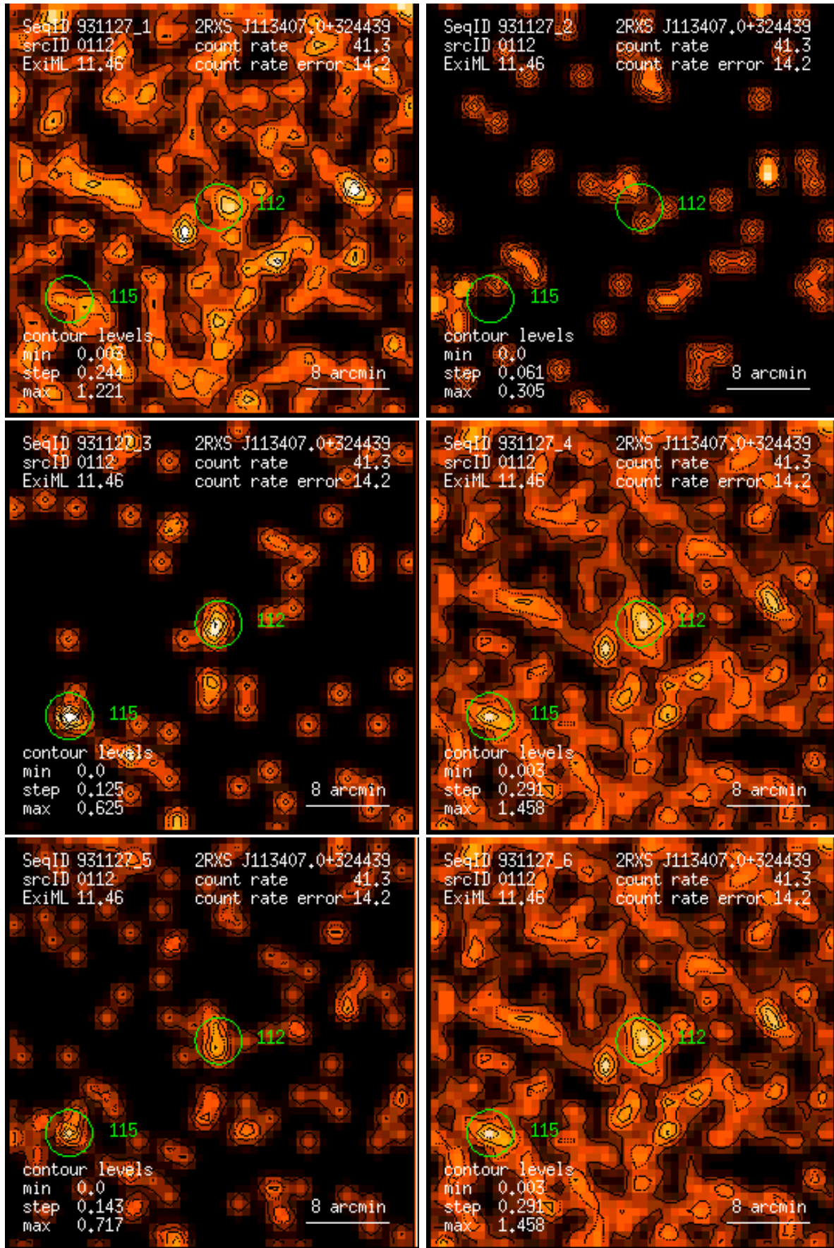
Figure 112: RASS 931127: detection 0112: band rate images, Gaussian filter: (1) PSPC channels 11 – 41, (2) 52 – 90, (3) 91 – 201, (4) 11 – 235, (5) 52 – 201, (6) 11 – 201. Broad band rates in counts/ks. Band rate contour levels in counts/ks/arcmin 2 .
