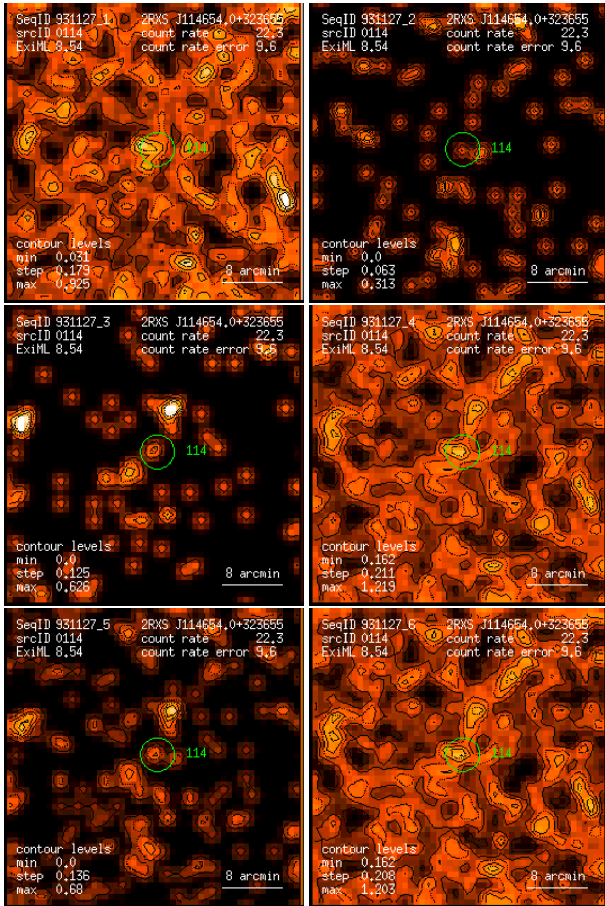
Figure 114: RASS 931127: detection 0114: band rate images, Gaussian filter: (1) PSPC channels 11 – 41, (2) 52 – 90, (3) 91 – 201, (4) 11 – 235, (5) 52 – 201, (6) 11 – 201. Broad band rates in counts/ks. Band rate contour levels in counts/ks/arcmin 2 .
