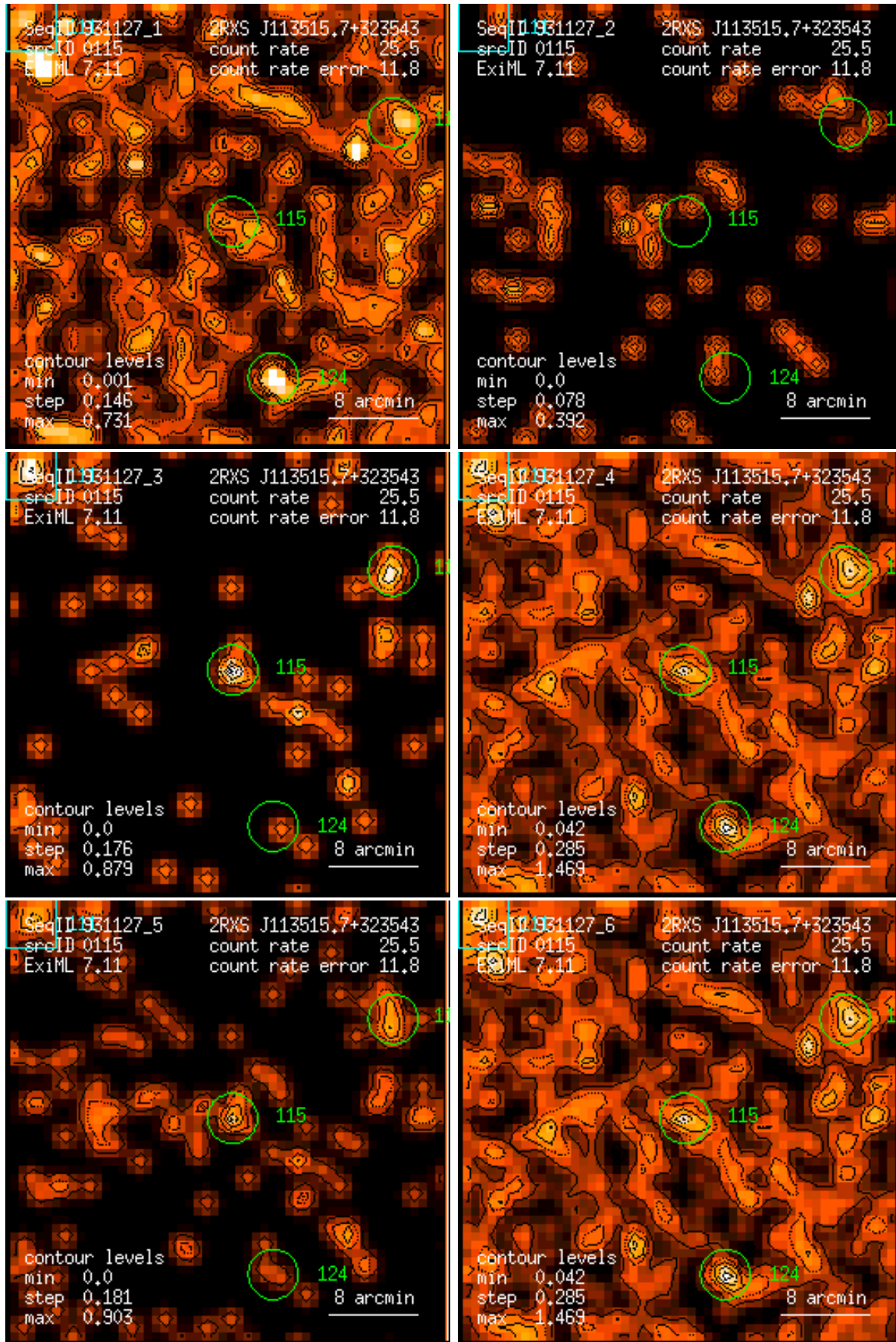
Figure 115: RASS 931127: detection 0115: band rate images, Gaussian filter: (1) PSPC channels 11 – 41, (2) 52 – 90, (3) 91 – 201, (4) 11 – 235, (5) 52 – 201, (6) 11 – 201. Broad band rates in counts/ks. Band rate contour levels in counts/ks/arcmin 2 .
