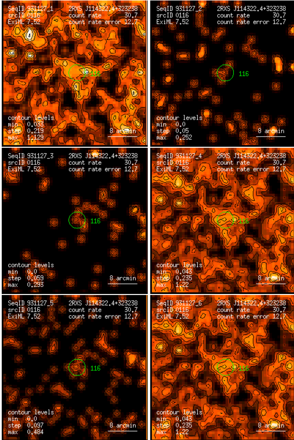
Figure 116: RASS 931127: detection 0116: band rate images, Gaussian filter: (1) PSPC channels 11 – 41, (2) 52 – 90, (3) 91 – 201, (4) 11 – 235, (5) 52 – 201, (6) 11 – 201. Broad band rates in counts/ks. Band rate contour levels in counts/ks/arcmin 2 .
