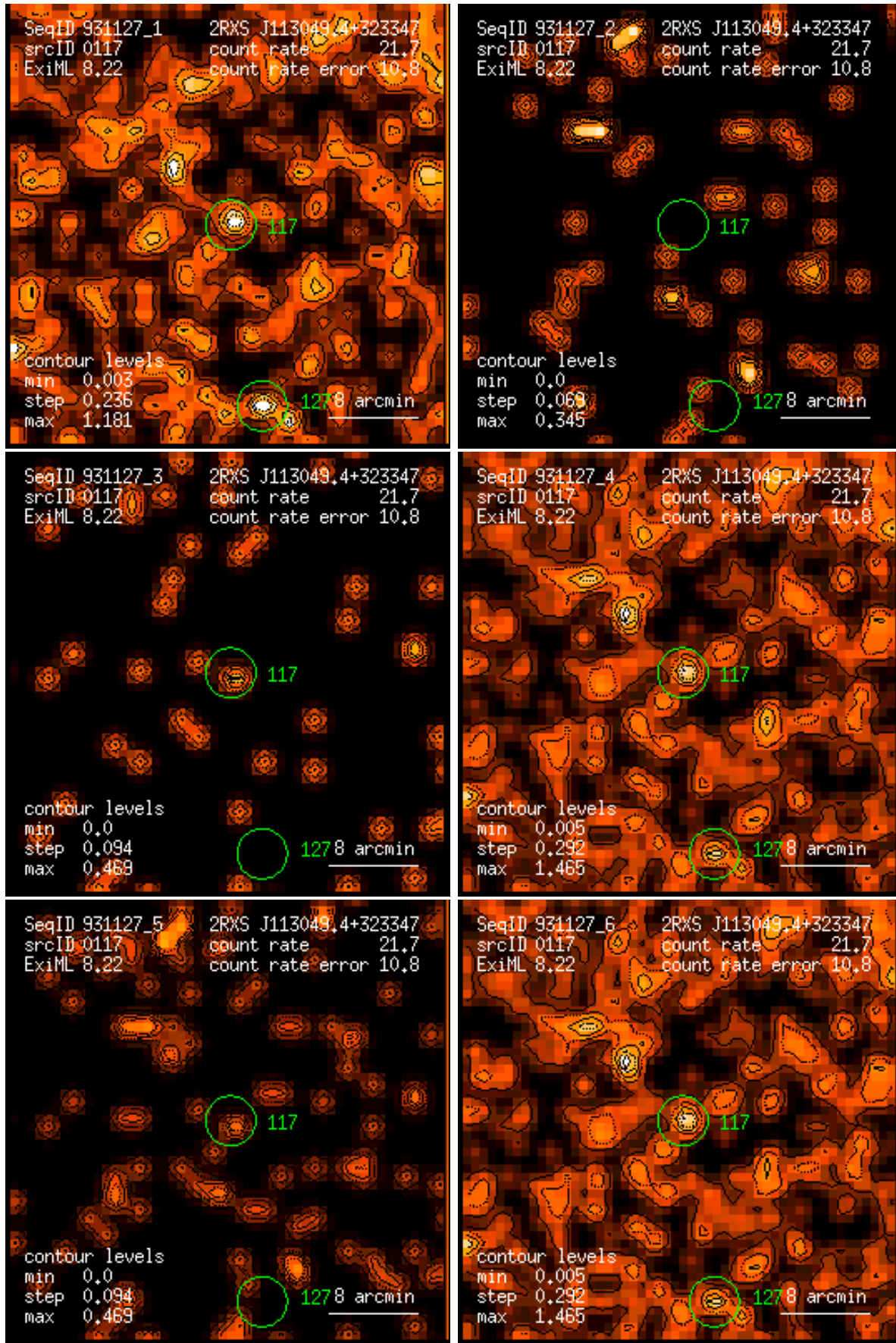
Figure 117: RASS 931127: detection 0117: band rate images, Gaussian filter: (1) PSPC channels 11 – 41, (2) 52 – 90, (3) 91 – 201, (4) 11 – 235, (5) 52 – 201, (6) 11 – 201. Broad band rates in counts/ks. Band rate contour levels in counts/ks/arcmin 2 .
