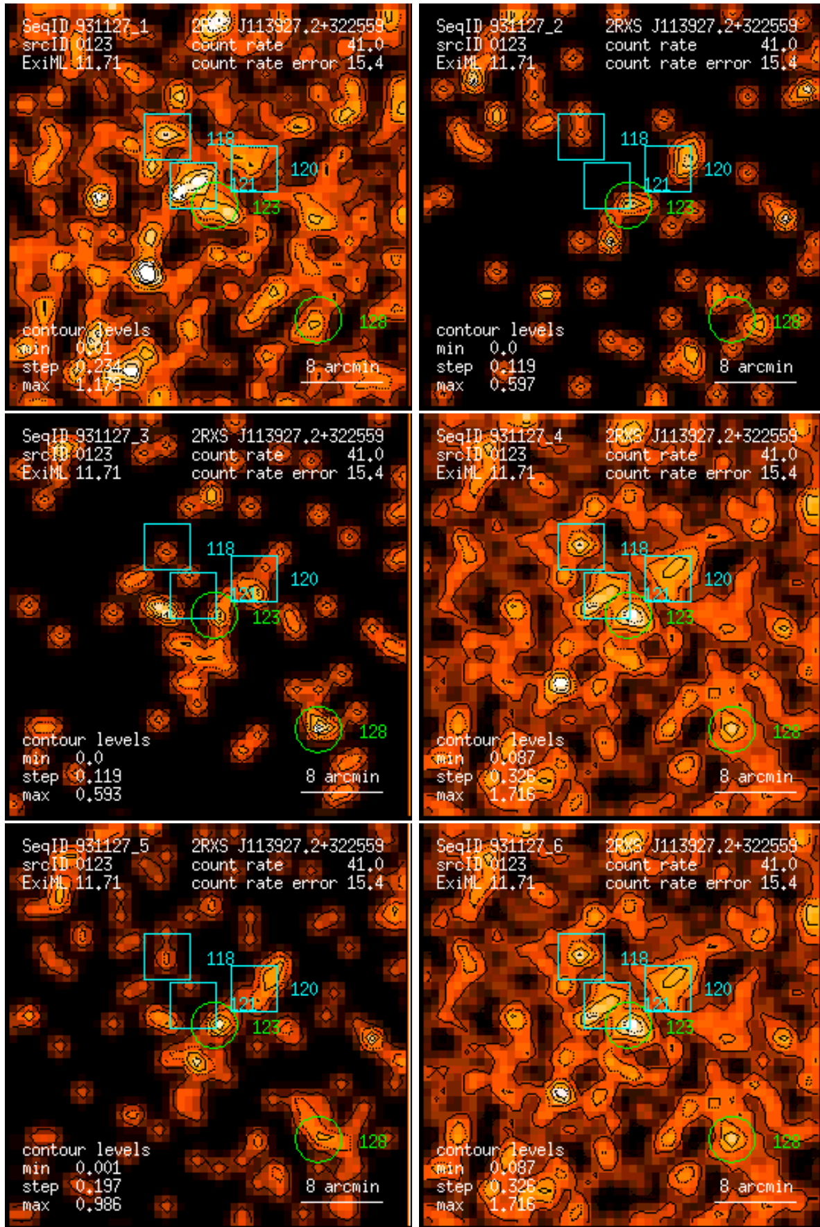
Figure 123: RASS 931127: detection 0123: band rate images, Gaussian filter: (1) PSPC channels 11 – 41, (2) 52 – 90, (3) 91 – 201, (4) 11 – 235, (5) 52 – 201, (6) 11 – 201. Broad band rates in counts/ks. Band rate contour levels in counts/ks/arcmin 2 .
