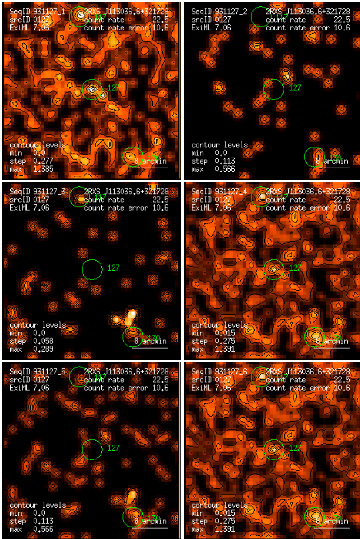
Figure 127: RASS 931127: detection 0127: band rate images, Gaussian filter: (1) PSPC channels 11 – 41, (2) 52 – 90, (3) 91 – 201, (4) 11 – 235, (5) 52 – 201, (6) 11 – 201. Broad band rates in counts/ks. Band rate contour levels in counts/ks/arcmin 2 .
