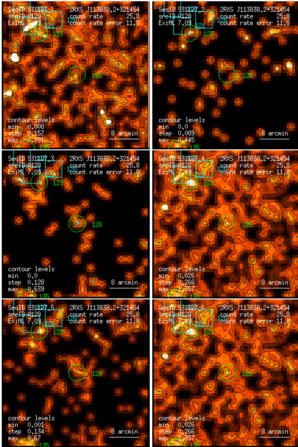
Figure 128: RASS 931127: detection 0128: band rate images, Gaussian filter: (1) PSPC channels 11 – 41, (2) 52 – 90, (3) 91 – 201, (4) 11 – 235, (5) 52 – 201, (6) 11 – 201. Broad band rates in counts/ks. Band rate contour levels in counts/ks/arcmin 2 .
