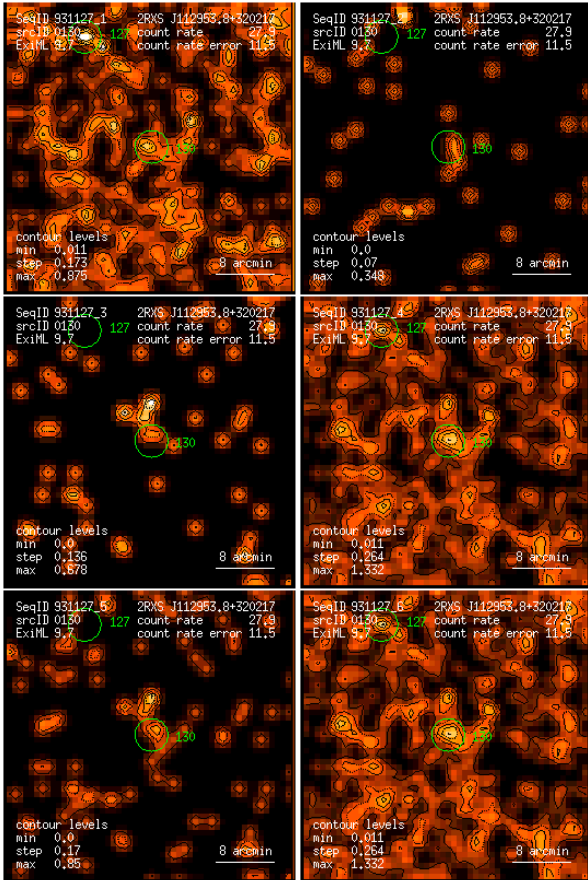
Figure 130: RASS 931127: detection 0130: band rate images, Gaussian filter: (1) PSPC channels 11 – 41, (2) 52 – 90, (3) 91 – 201, (4) 11 – 235, (5) 52 – 201, (6) 11 – 201. Broad band rates in counts/ks. Band rate contour levels in counts/ks/arcmin 2 .
