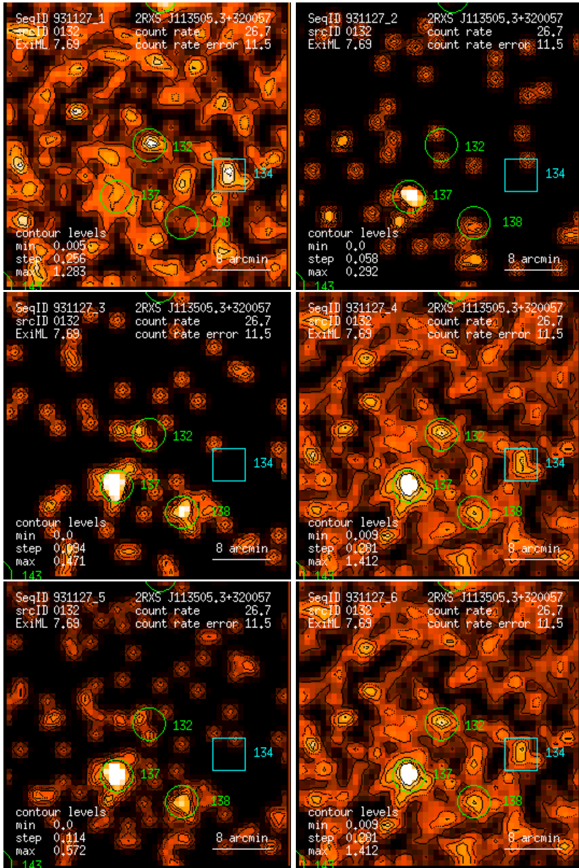
Figure 132: RASS 931127: detection 0132: band rate images, Gaussian filter: (1) PSPC channels 11 – 41, (2) 52 – 90, (3) 91 – 201, (4) 11 – 235, (5) 52 – 201, (6) 11 – 201. Broad band rates in counts/ks. Band rate contour levels in counts/ks/arcmin 2 .
