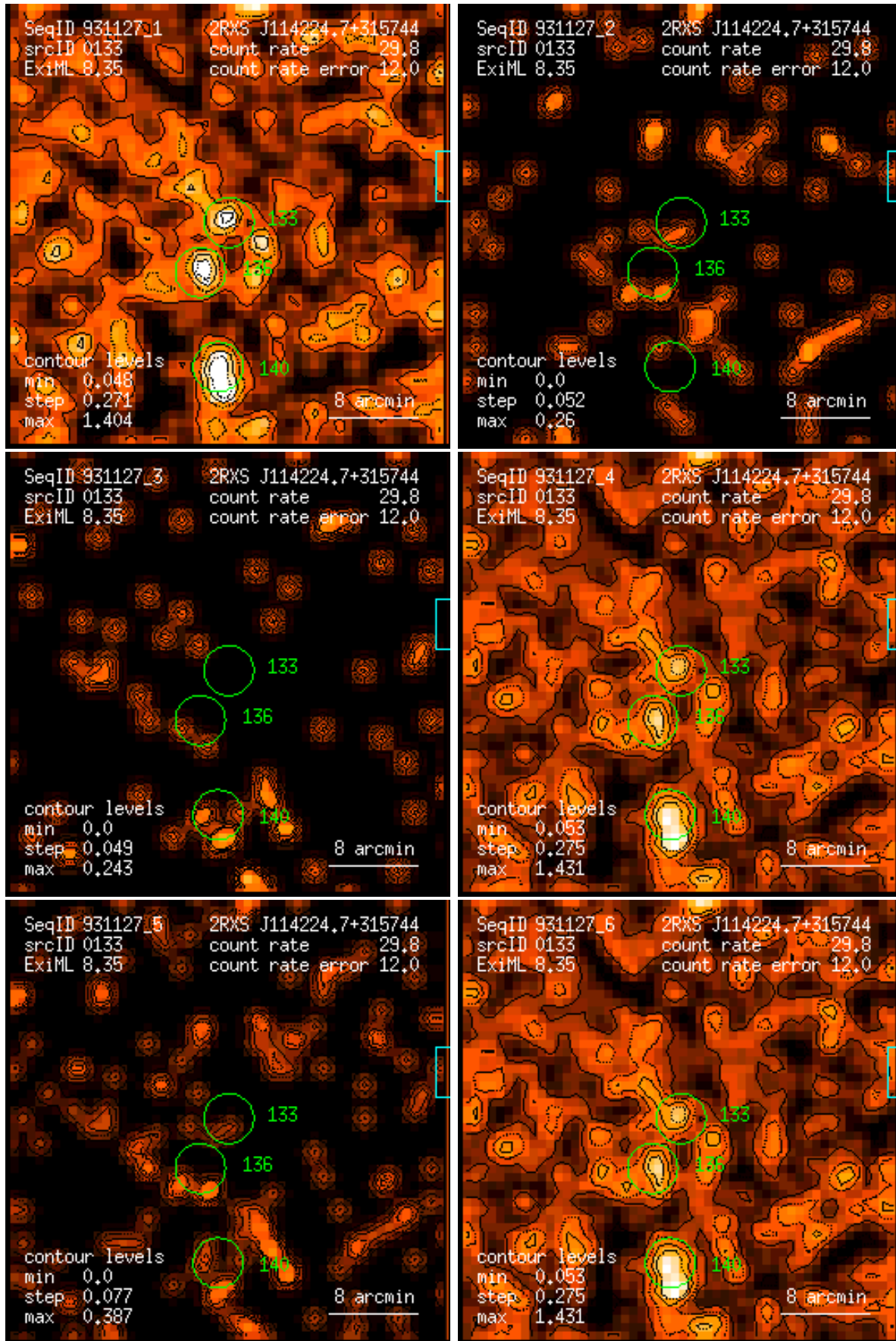
Figure 133: RASS 931127: detection 0133: band rate images, Gaussian filter: (1) PSPC channels 11 – 41, (2) 52 – 90, (3) 91 – 201, (4) 11 – 235, (5) 52 – 201, (6) 11 – 201. Broad band rates in counts/ks. Band rate contour levels in counts/ks/arcmin 2 .
