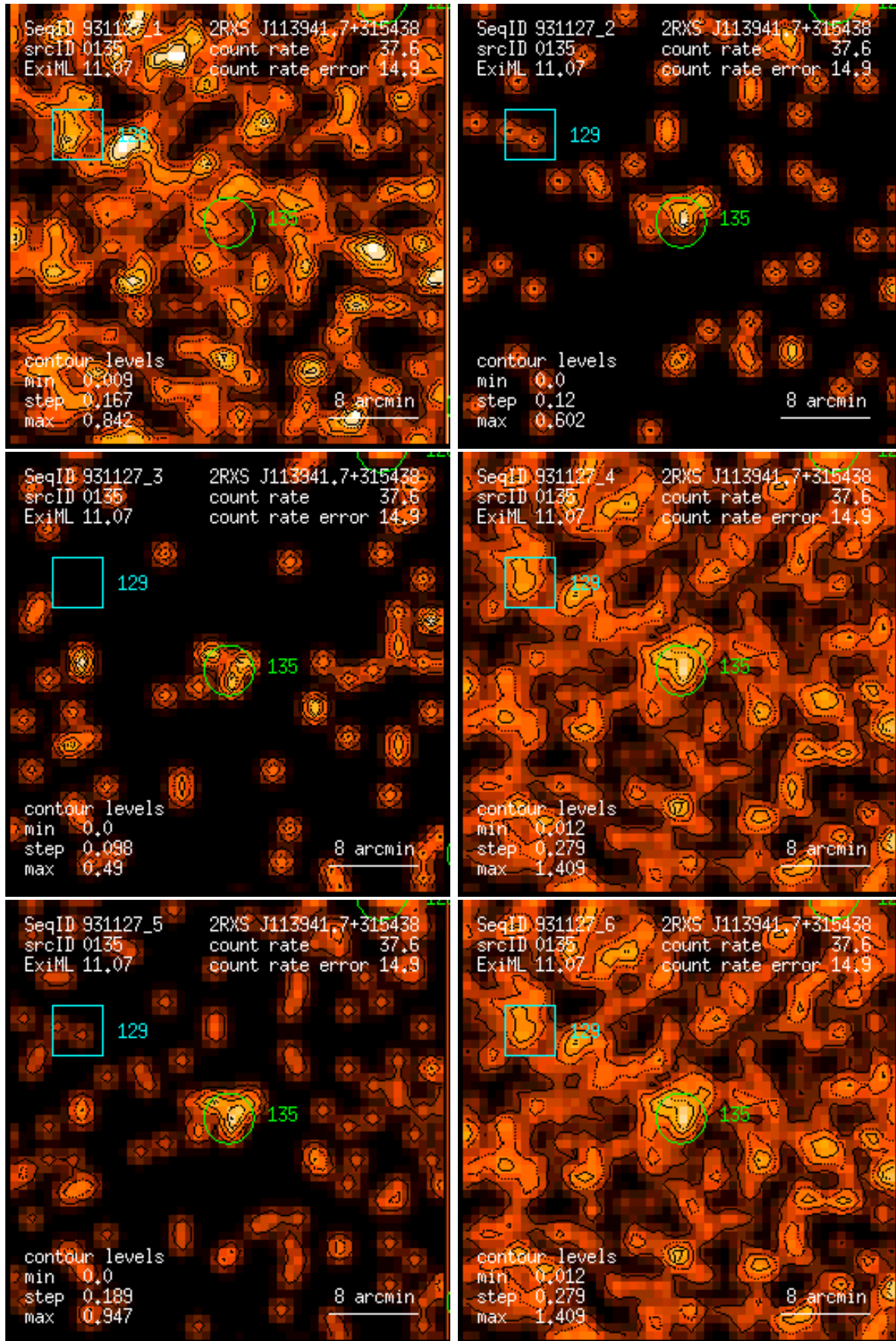
Figure 135: RASS 931127: detection 0135: band rate images, Gaussian filter: (1) PSPC channels 11 – 41, (2) 52 – 90, (3) 91 – 201, (4) 11 – 235, (5) 52 – 201, (6) 11 – 201. Broad band rates in counts/ks. Band rate contour levels in counts/ks/arcmin 2 .
