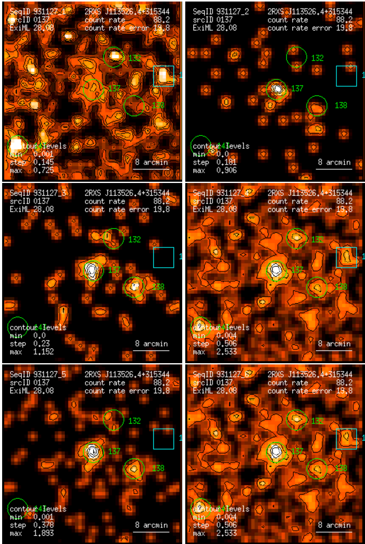
Figure 137: RASS 931127: detection 0137: band rate images, Gaussian filter: (1) PSPC channels 11 – 41, (2) 52 – 90, (3) 91 – 201, (4) 11 – 235, (5) 52 – 201, (6) 11 – 201. Broad band rates in counts/ks. Band rate contour levels in counts/ks/arcmin 2 .
