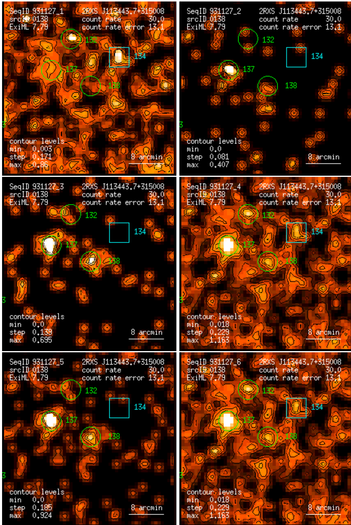
Figure 138: RASS 931127: detection 0138: band rate images, Gaussian filter: (1) PSPC channels 11 – 41, (2) 52 – 90, (3) 91 – 201, (4) 11 – 235, (5) 52 – 201, (6) 11 – 201. Broad band rates in counts/ks. Band rate contour levels in counts/ks/arcmin 2 .
