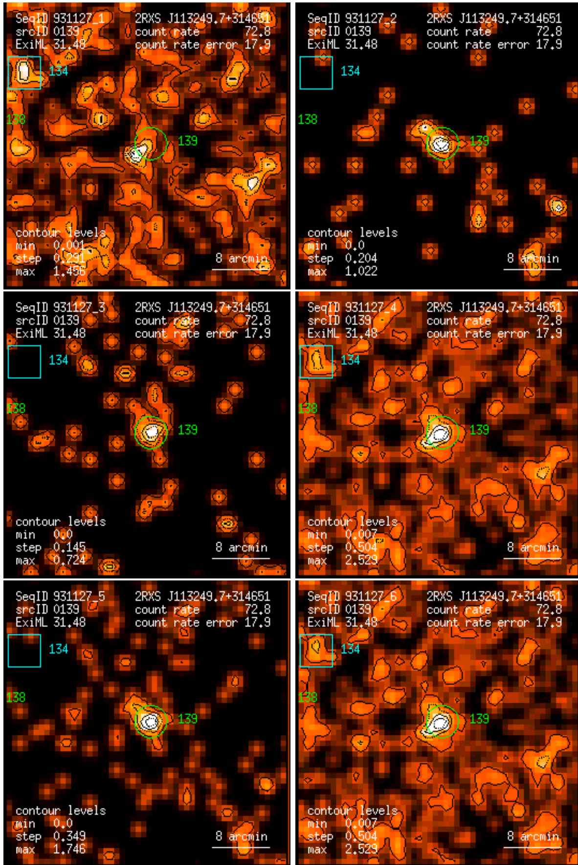
Figure 139: RASS 931127: detection 0139: band rate images, Gaussian filter: (1) PSPC channels 11 – 41, (2) 52 – 90, (3) 91 – 201, (4) 11 – 235, (5) 52 – 201, (6) 11 – 201. Broad band rates in counts/ks. Band rate contour levels in counts/ks/arcmin 2 .
