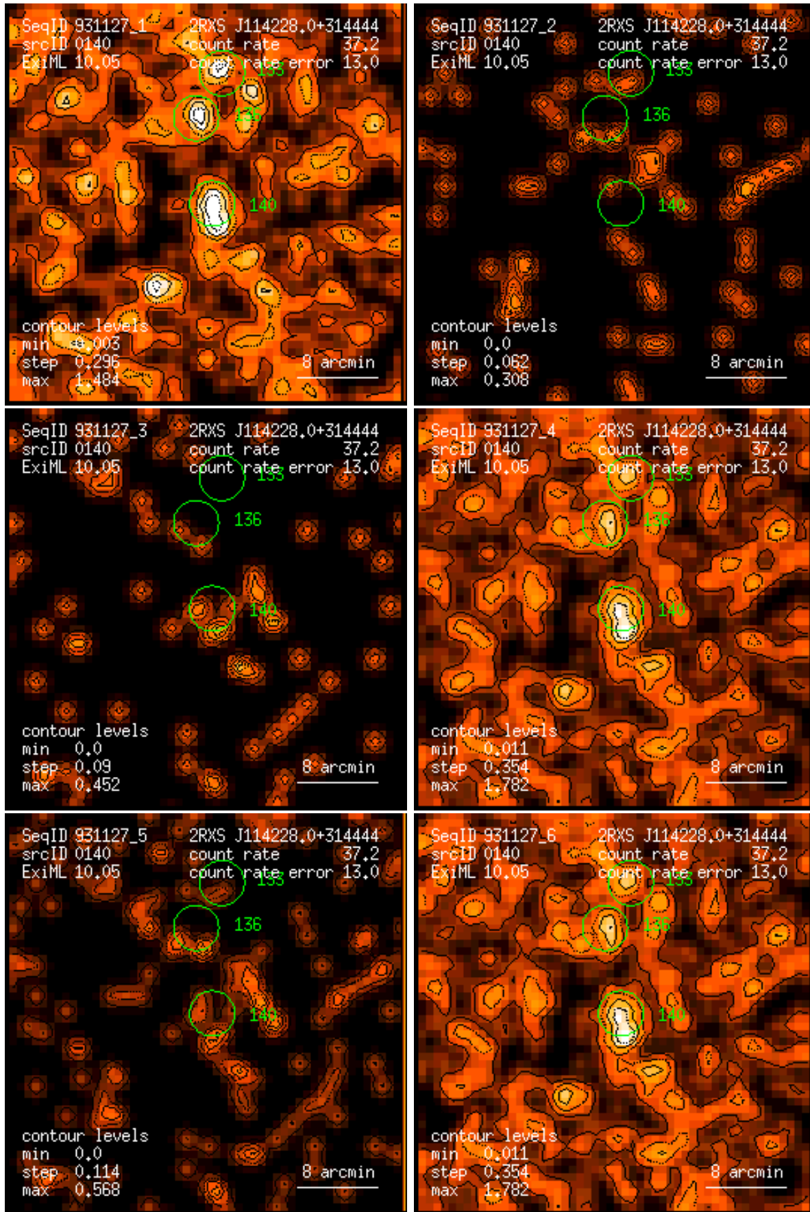
Figure 140: RASS 931127: detection 0140: band rate images, Gaussian filter: (1) PSPC channels 11 – 41, (2) 52 – 90, (3) 91 – 201, (4) 11 – 235, (5) 52 – 201, (6) 11 – 201. Broad band rates in counts/ks. Band rate contour levels in counts/ks/arcmin 2 .
