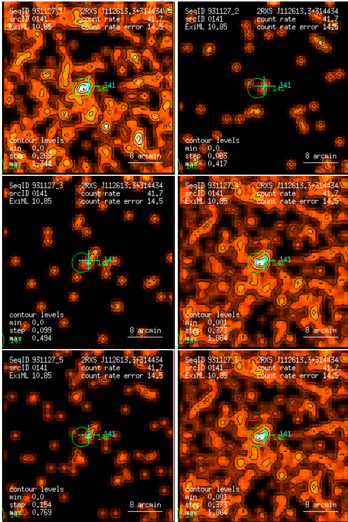
Figure 141: RASS 931127: detection 0141: band rate images, Gaussian filter: (1) PSPC channels 11 – 41, (2) 52 – 90, (3) 91 – 201, (4) 11 – 235, (5) 52 – 201, (6) 11 – 201. Broad band rates in counts/ks. Band rate contour levels in counts/ks/arcmin 2 .
