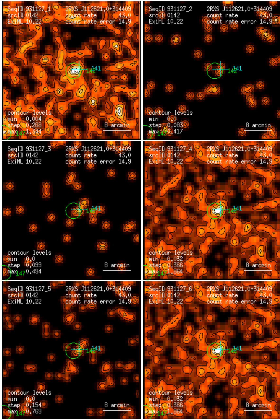
Figure 142: RASS 931127: detection 0142: band rate images, Gaussian filter: (1) PSPC channels 11 – 41, (2) 52 – 90, (3) 91 – 201, (4) 11 – 235, (5) 52 – 201, (6) 11 – 201. Broad band rates in counts/ks. Band rate contour levels in counts/ks/arcmin 2 .
