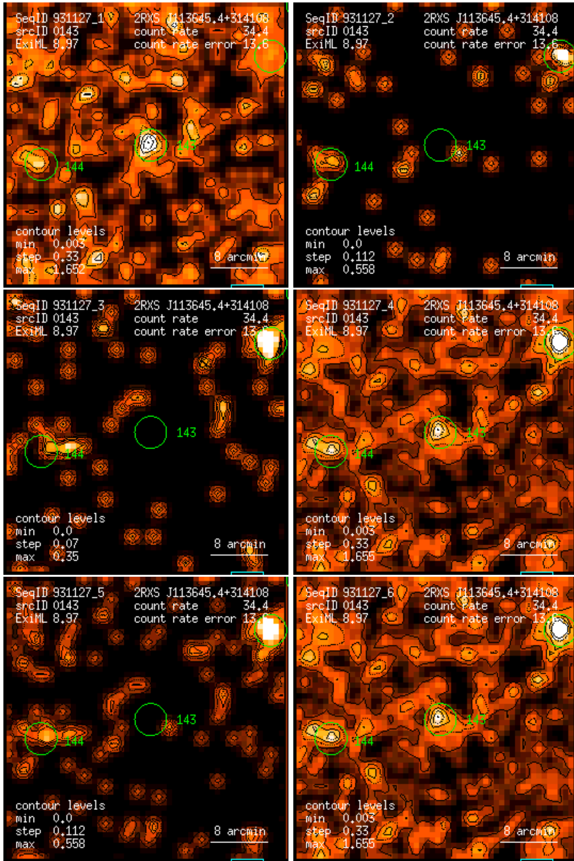
Figure 143: RASS 931127: detection 0143: band rate images, Gaussian filter: (1) PSPC channels 11 – 41, (2) 52 – 90, (3) 91 – 201, (4) 11 – 235, (5) 52 – 201, (6) 11 – 201. Broad band rates in counts/ks. Band rate contour levels in counts/ks/arcmin 2 .
