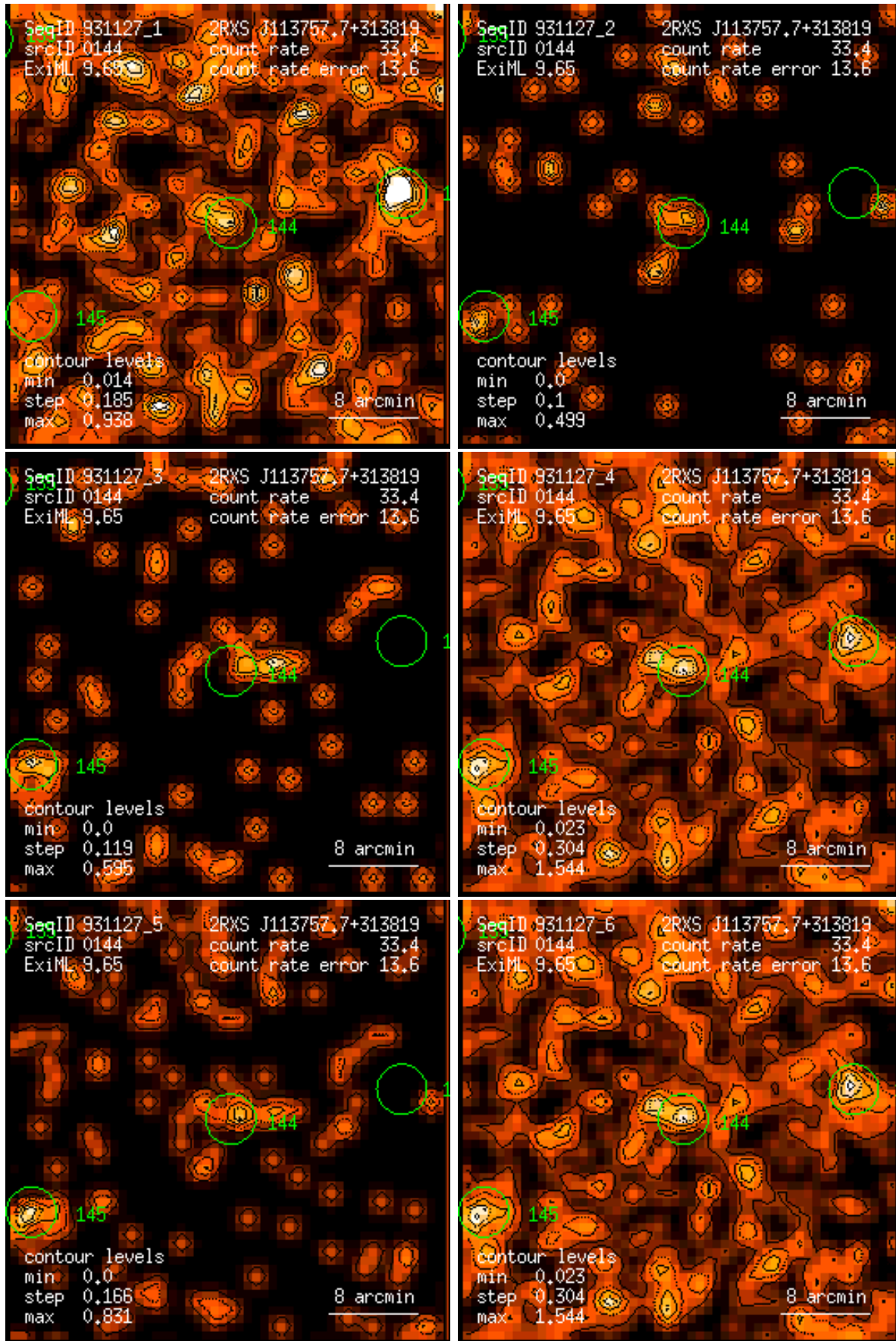
Figure 144: RASS 931127: detection 0144: band rate images, Gaussian filter: (1) PSPC channels 11 – 41, (2) 52 – 90, (3) 91 – 201, (4) 11 – 235, (5) 52 – 201, (6) 11 – 201. Broad band rates in counts/ks. Band rate contour levels in counts/ks/arcmin 2 .
