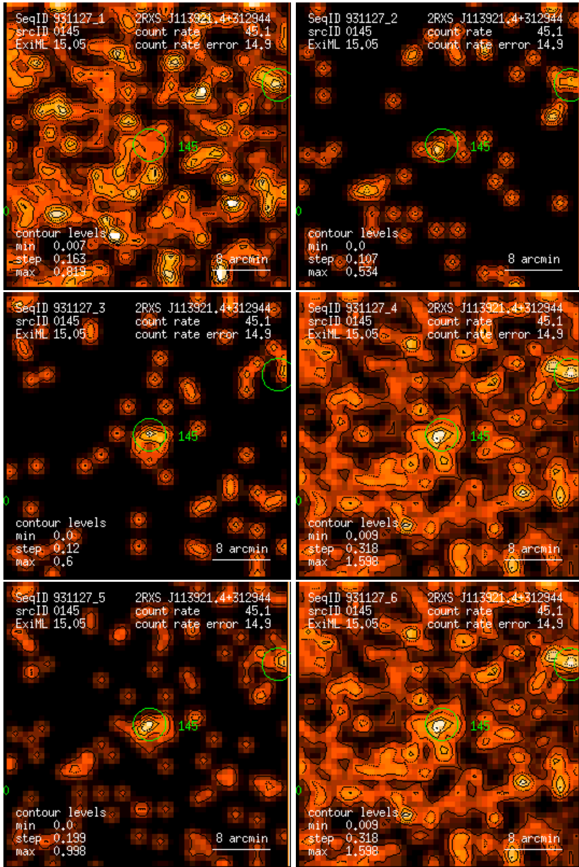
Figure 145: RASS 931127: detection 0145: band rate images, Gaussian filter: (1) PSPC channels 11 – 41, (2) 52 – 90, (3) 91 – 201, (4) 11 – 235, (5) 52 – 201, (6) 11 – 201. Broad band rates in counts/ks. Band rate contour levels in counts/ks/arcmin 2 .
