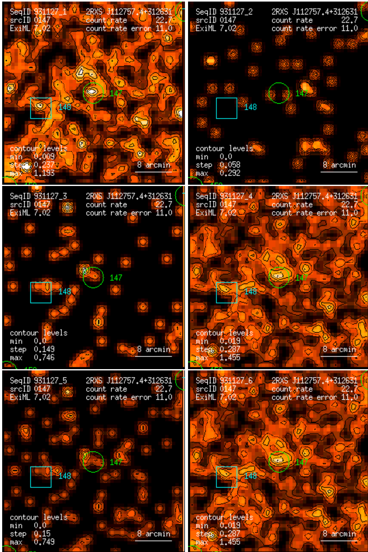
Figure 147: RASS 931127: detection 0147: band rate images, Gaussian filter: (1) PSPC channels 11 – 41, (2) 52 – 90, (3) 91 – 201, (4) 11 – 235, (5) 52 – 201, (6) 11 – 201. Broad band rates in counts/ks. Band rate contour levels in counts/ks/arcmin 2 .
