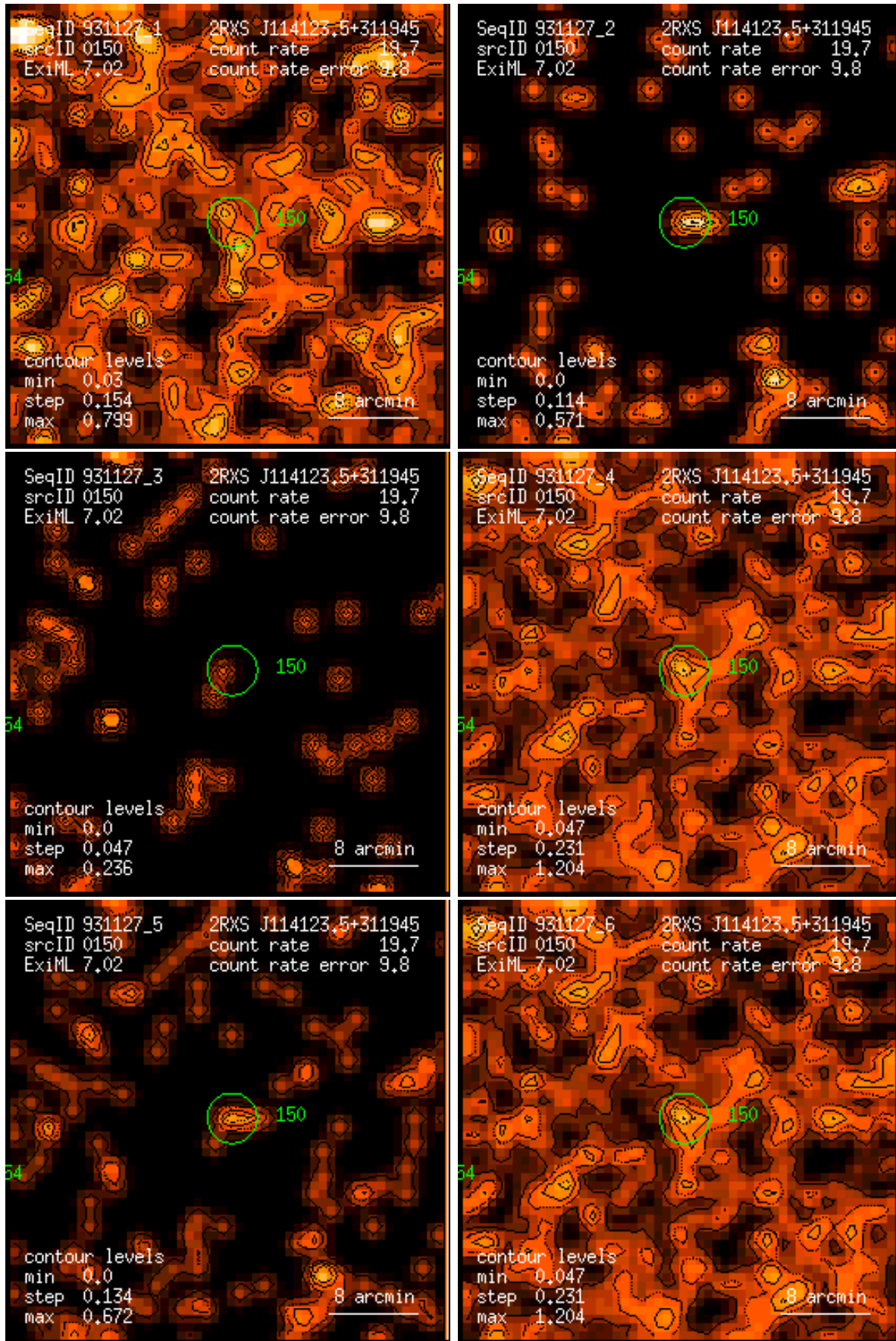
Figure 150: RASS 931127: detection 0150: band rate images, Gaussian filter: (1) PSPC channels 11 – 41, (2) 52 – 90, (3) 91 – 201, (4) 11 – 235, (5) 52 – 201, (6) 11 – 201. Broad band rates in counts/ks. Band rate contour levels in counts/ks/arcmin 2 .
