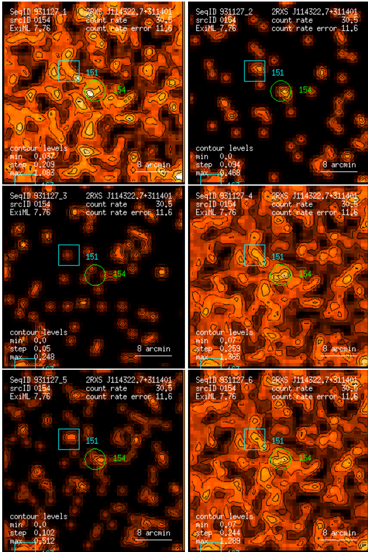
Figure 154: RASS 931127: detection 0154: band rate images, Gaussian filter: (1) PSPC channels 11 – 41, (2) 52 – 90, (3) 91 – 201, (4) 11 – 235, (5) 52 – 201, (6) 11 – 201. Broad band rates in counts/ks. Band rate contour levels in counts/ks/arcmin 2 .
