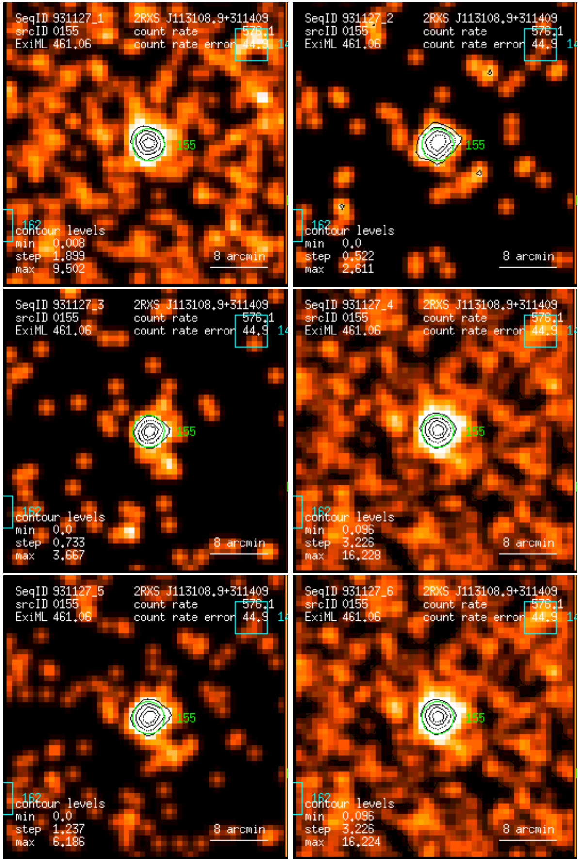
Figure 155: RASS 931127: detection 0155: band rate images, Gaussian filter: (1) PSPC channels 11 – 41, (2) 52 – 90, (3) 91 – 201, (4) 11 – 235, (5) 52 – 201, (6) 11 – 201. Broad band rates in counts/ks. Band rate contour levels in counts/ks/arcmin 2 .
