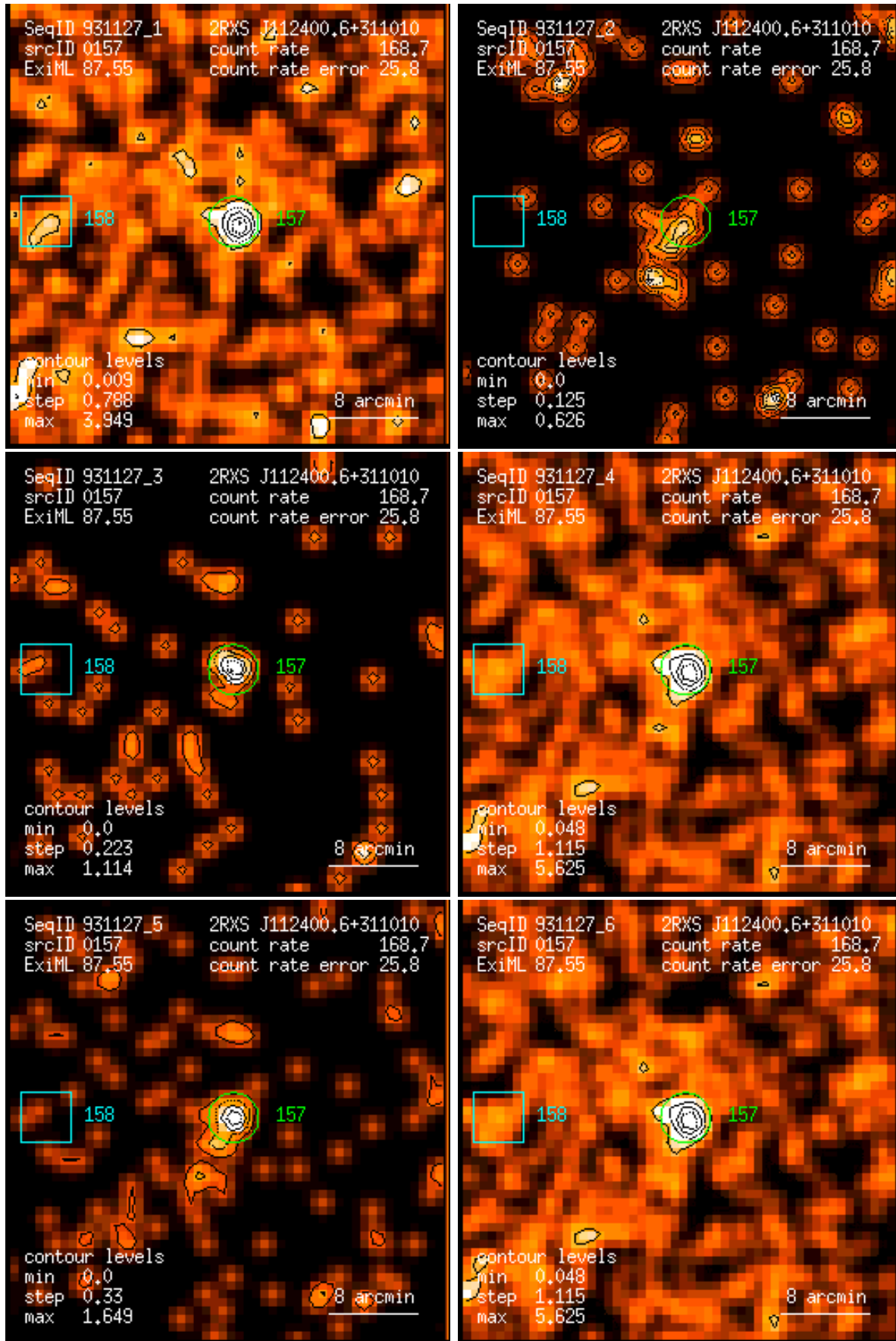
Figure 157: RASS 931127: detection 0157: band rate images, Gaussian filter: (1) PSPC channels 11 – 41, (2) 52 – 90, (3) 91 – 201, (4) 11 – 235, (5) 52 – 201, (6) 11 – 201. Broad band rates in counts/ks. Band rate contour levels in counts/ks/arcmin 2 .
